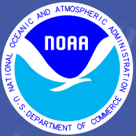
Weather Forecast for Thursday, August 21, 2008 DOC/NOAA/NWS/NCEP/Hydrometeorological Prediction Center Prepared by Engelman based on HPC, SPC, and TPC forecasts.
