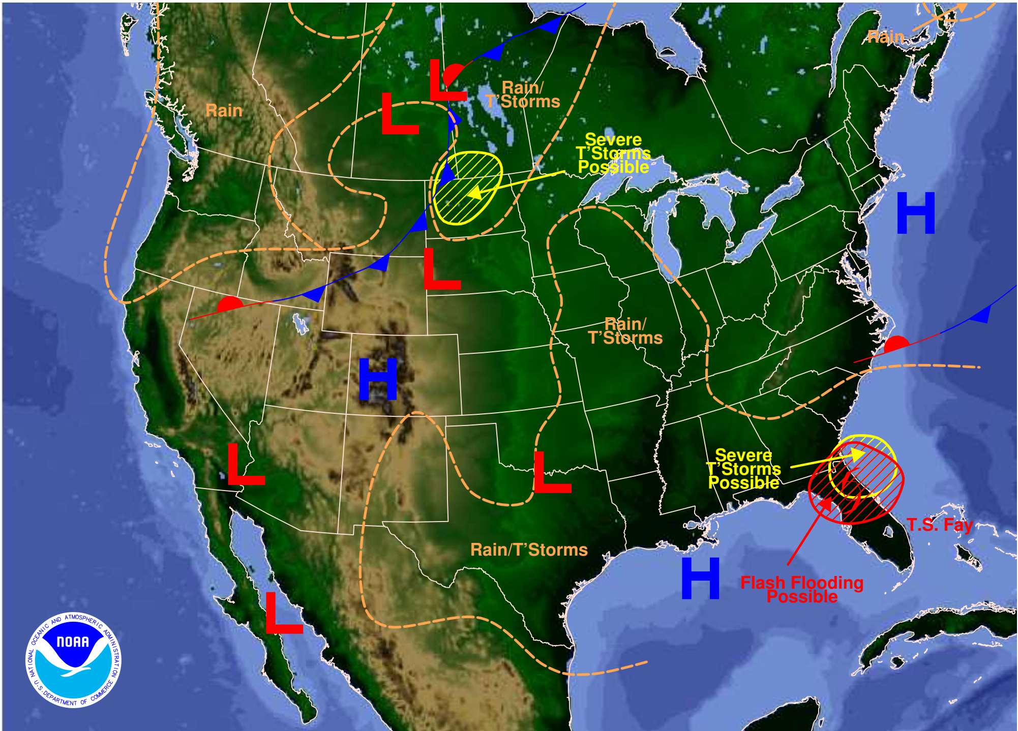
Weather Forecast for Thursday, August 21, 2008 DOC/NOAA/NWS/NCEP/Hydrometeorological Prediction Center Prepared by Engelman based on HPC, SPC, and TPC forecasts.
