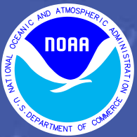
Weather Forecast for Friday, July 04, 2008 DOC/NOAA/NWS/NCEP/Hydrometeorological Prediction Center Prepared by Kost based on HPC, SPC, and TPC forecasts.
