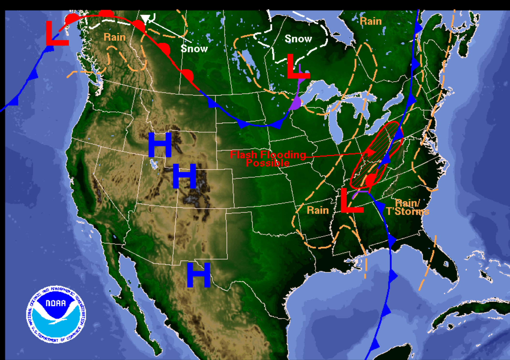
Weather Forecast for Tuesday, October 23, 2007 DOC/NOAA/NWS/NCEP/Hydrometeorological Prediction Center Prepared by Rubin-Oster based on HPC, SPC, and TPC forecasts.
