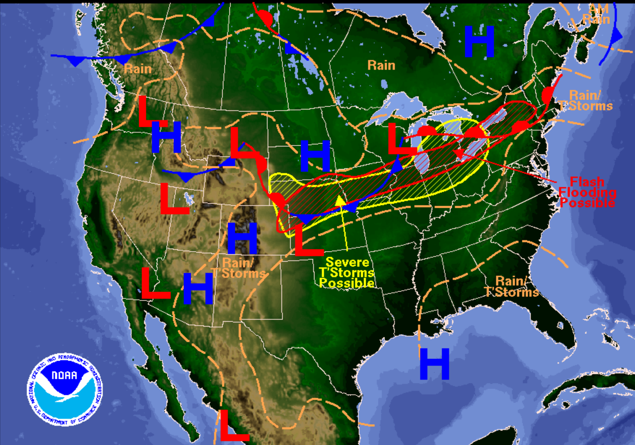
Weather Forecast for Tuesday, August 07, 2007 DOC/NOAA/NWS/NCEP/Hydrometeorological Prediction Center Prepared by Fracasso based on HPC, SPC, and TPC forecasts.
