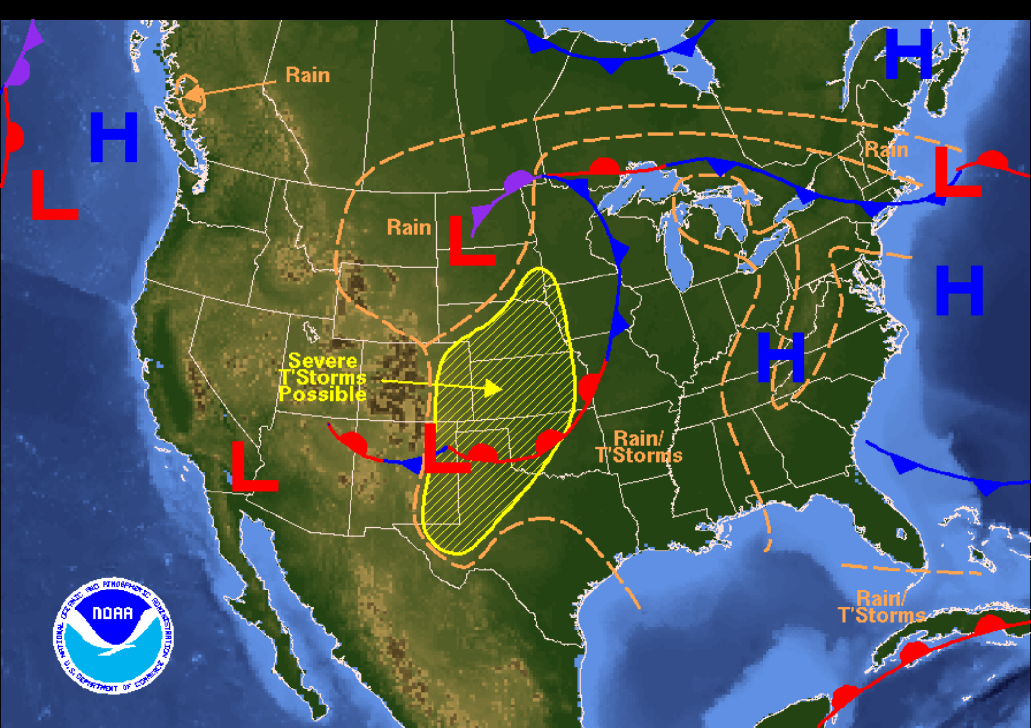
Weather Forecast for Thursday, May 31, 2007 DOC/NOAA/NWS/NCEP/Hydrometeorological Prediction Center Prepared by Fracasso based on HPC, SPC, and TPC forecasts.
