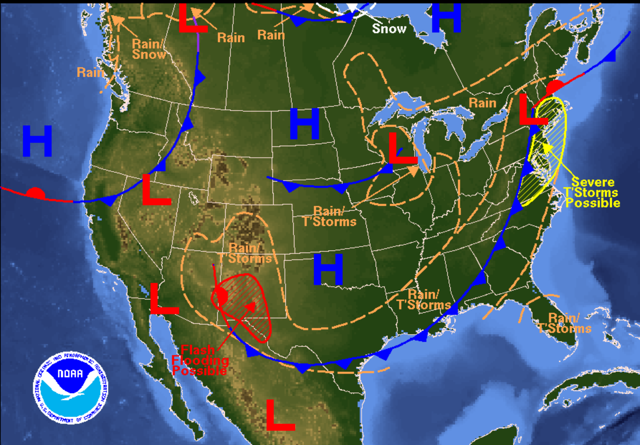
Weather Forecast for Wednesday, May 16, 2007 DOC/NOAA/NWS/NCEP/Hydrometeorological Prediction Center Prepared by Pereira based on HPC, SPC, and TPC forecasts.
