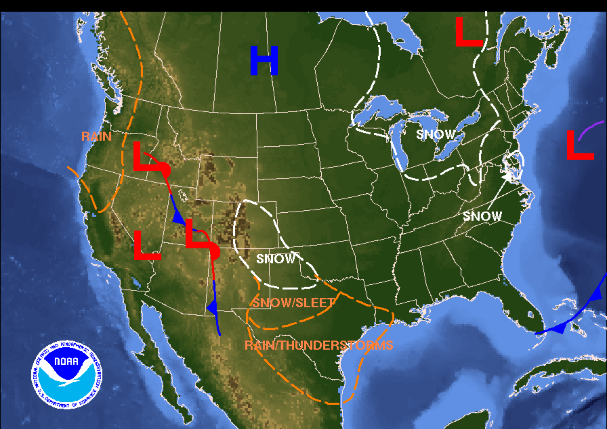
Weather Forecast for Saturday, April 07, 2007 DOC/NOAA/NWS/NCEP/Hydrometeorological Prediction Center Prepared by HEDGE based on HPC, SPC, and TPC forecasts.
