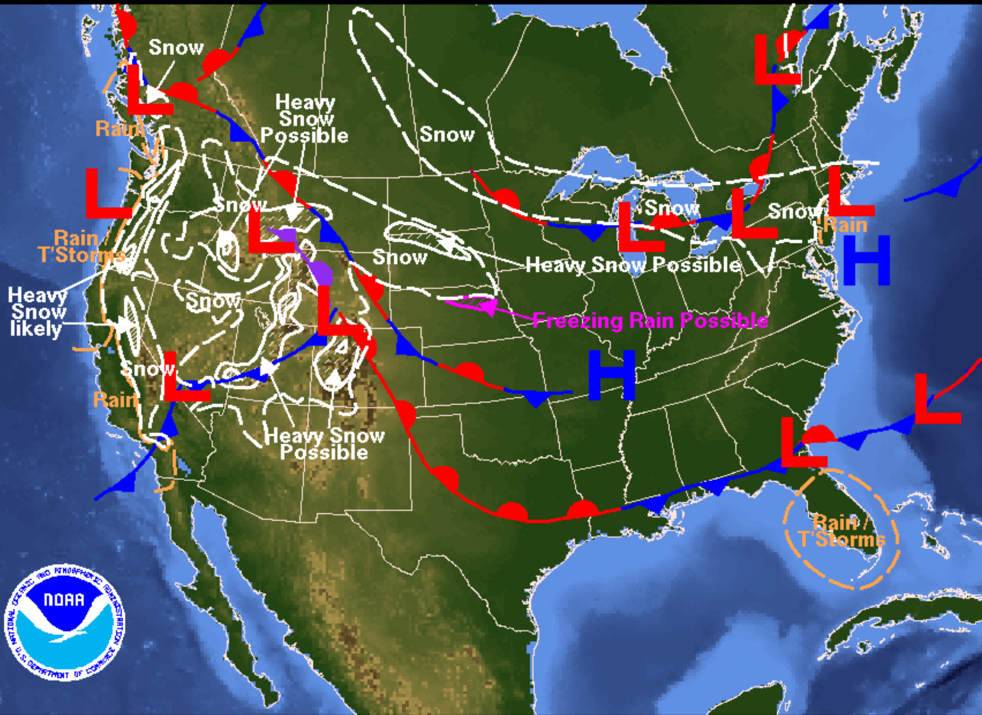
Weather Forecast for Tuesday, February 27, 2007 DOC/NOAA/NWS/NCEP/Hydrometeorological Prediction Center Prepared by Kong based on HPC, SPC, and TPC forecasts.
