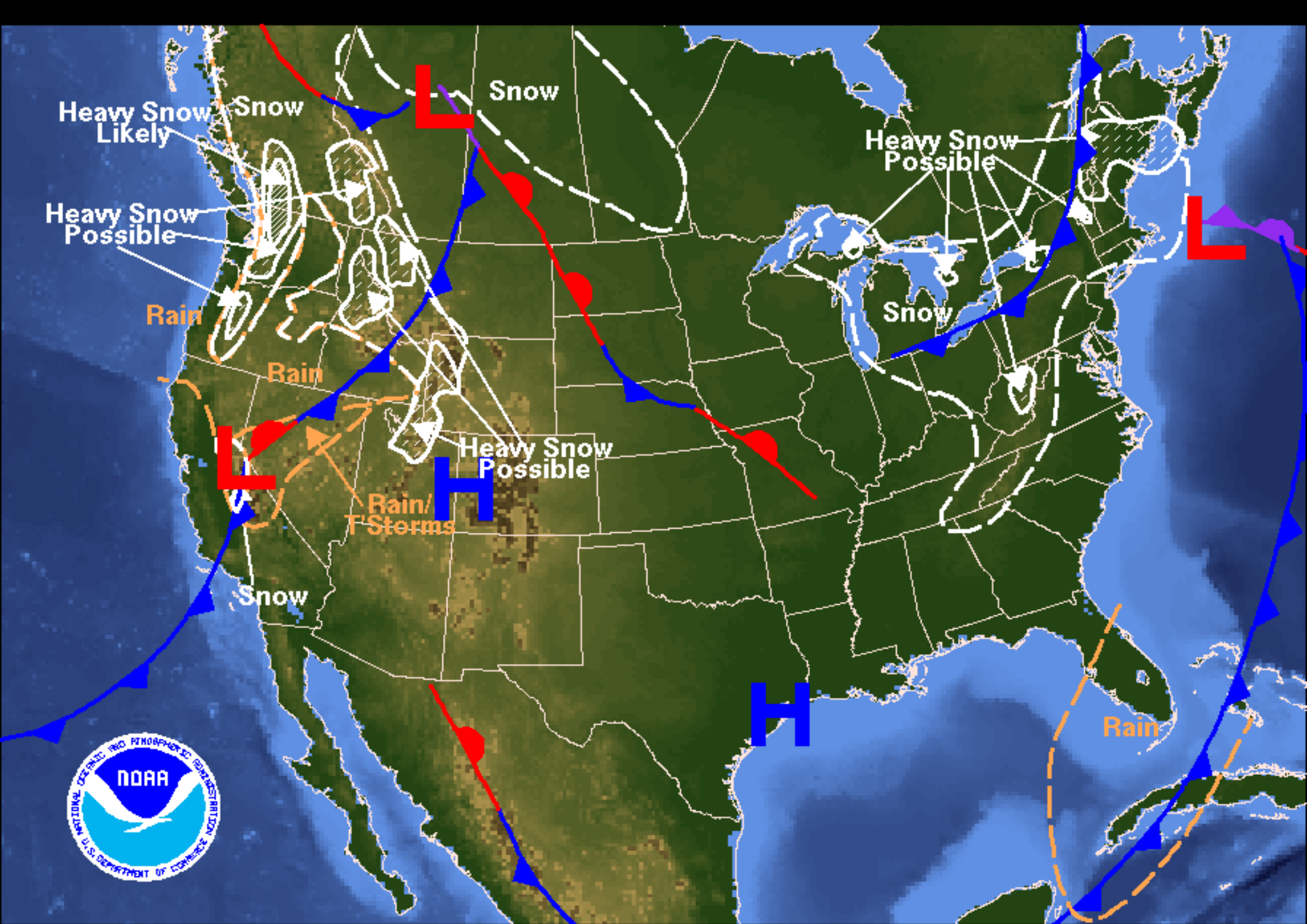
Weather Forecast for Sunday, February 18, 2007 DOC/NOAA/NWS/NCEP/Hydrometeorological Prediction Center Prepared by Rubin-Oster based on HPC, SPC, and TPC forecasts.
