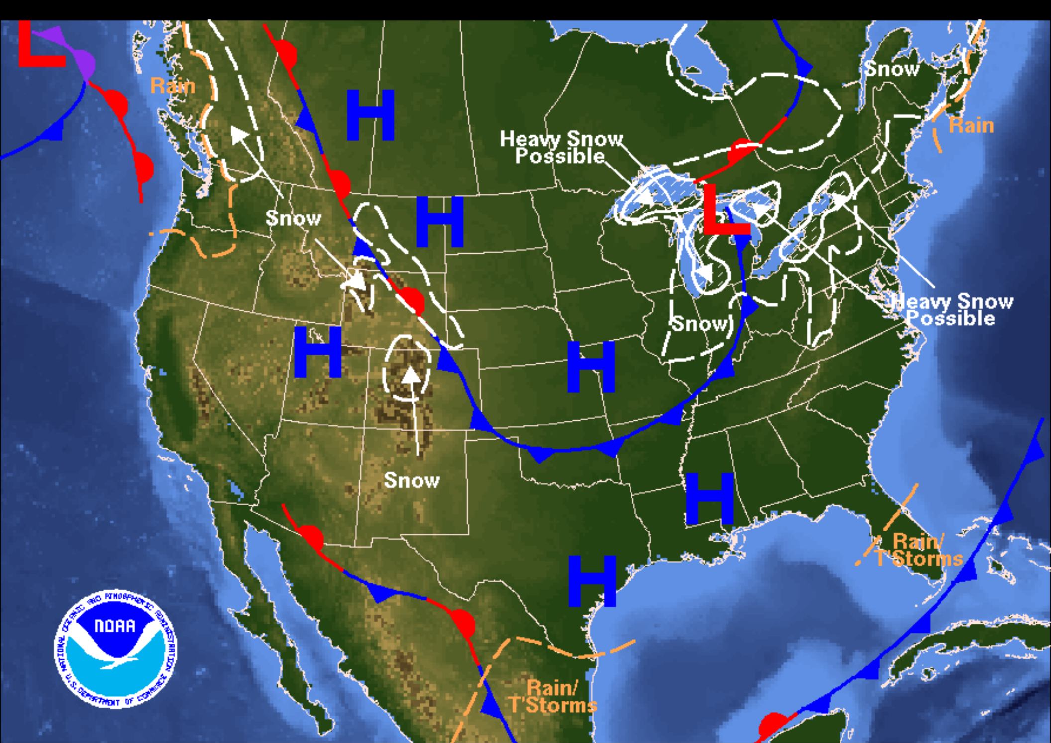
Weather Forecast for Saturday, February 03, 2007 DOC/NOAA/NWS/NCEP/Hydrometeorological Prediction Center Prepared by Otto based on HPC, SPC, and TPC forecasts.
