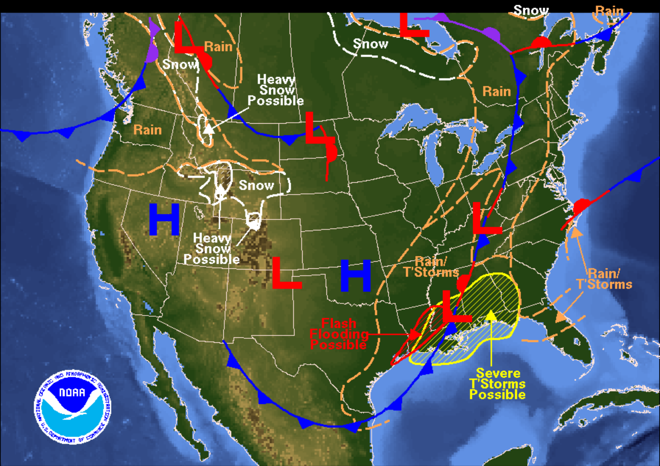
Weather Forecast for Thursday, October 19, 2006 DOC/NOAA/NWS/NCEP/Hydrometeorological Prediction Center Prepared by Trimarco based on HPC, SPC, and TPC forecasts.
