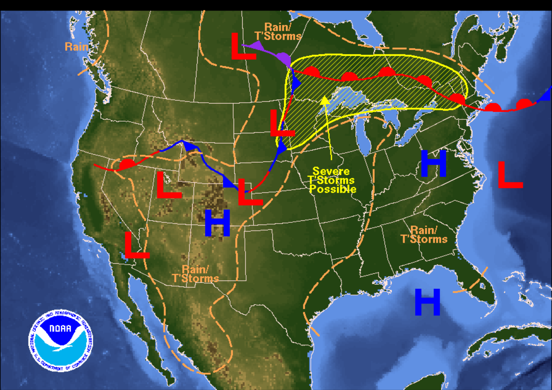
Weather Forecast for Monday, July 31, 2006 DOC/NOAA/NWS/NCEP/Hydrometeorological Prediction Center Prepared by Scheck based on HPC, SPC, and TPC forecasts.
