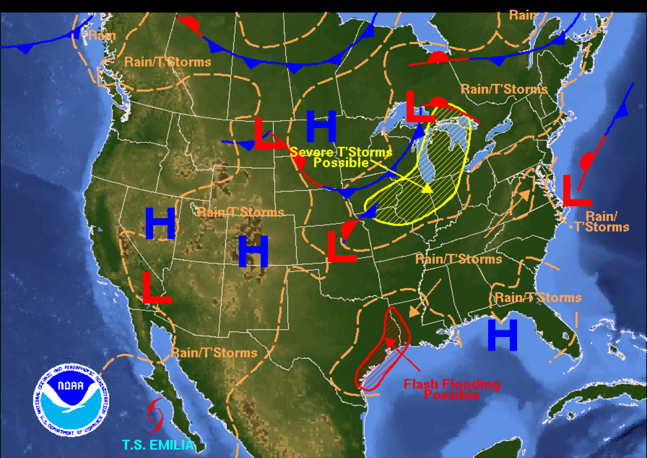
Weather Forecast for Wednesday, July 26, 2006 DOC/NOAA/NWS/NCEP/Hydrometeorological Prediction Center Prepared by Bell based on HPC, SPC, and TPC forecasts.
