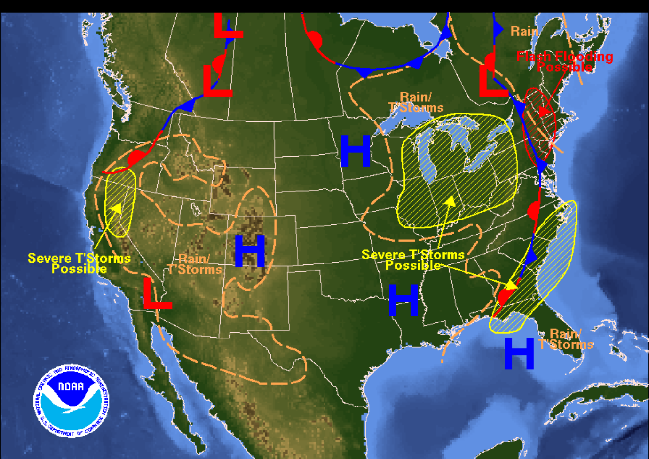
Weather Forecast for Wednesday, June 28, 2006 DOC/NOAA/NWS/NCEP/Hydrometeorological Prediction Center Prepared by Fries based on HPC, SPC, and TPC forecasts.
