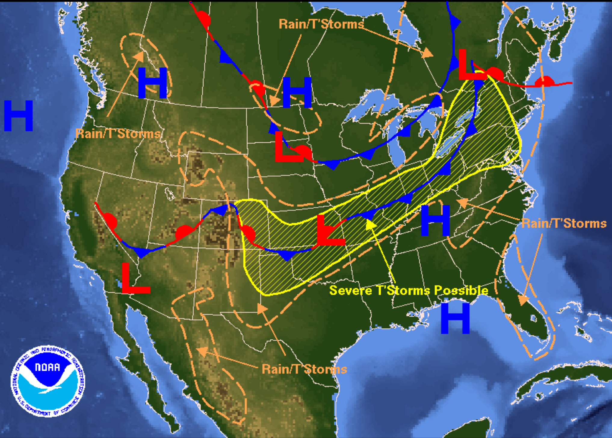
Weather Forecast for Thursday, June 22, 2006 DOC/NOAA/NWS/NCEP/Hydrometeorological Prediction Center Prepared by Oravec based on HPC, SPC, and TPC forecasts.
