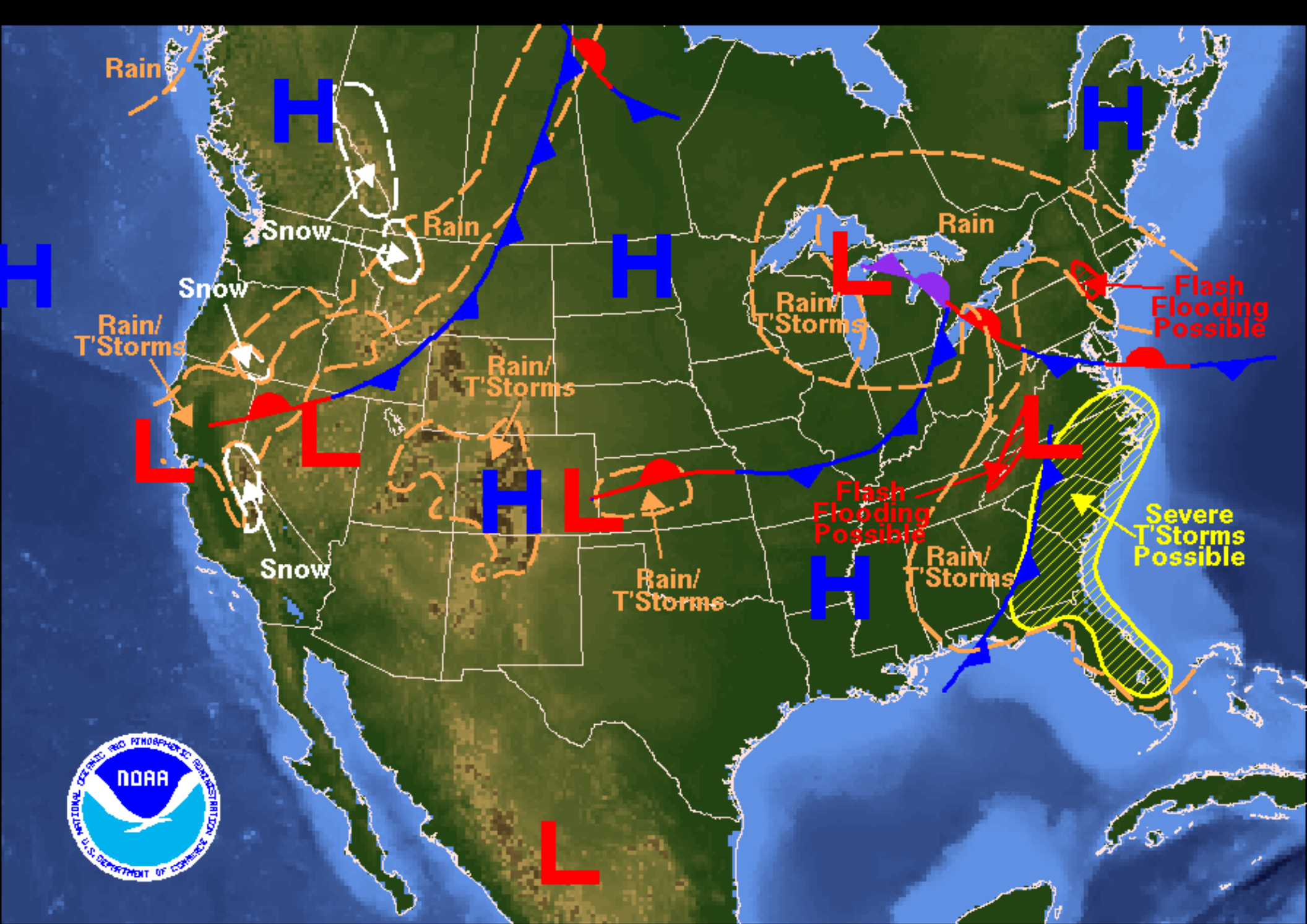
Weather Forecast for Saturday, April 22, 2006 DOC/NOAA/NWS/NCEP/Hydrometeorological Prediction Center Prepared by Trimarco based on HPC, SPC, and TPC forecasts.
