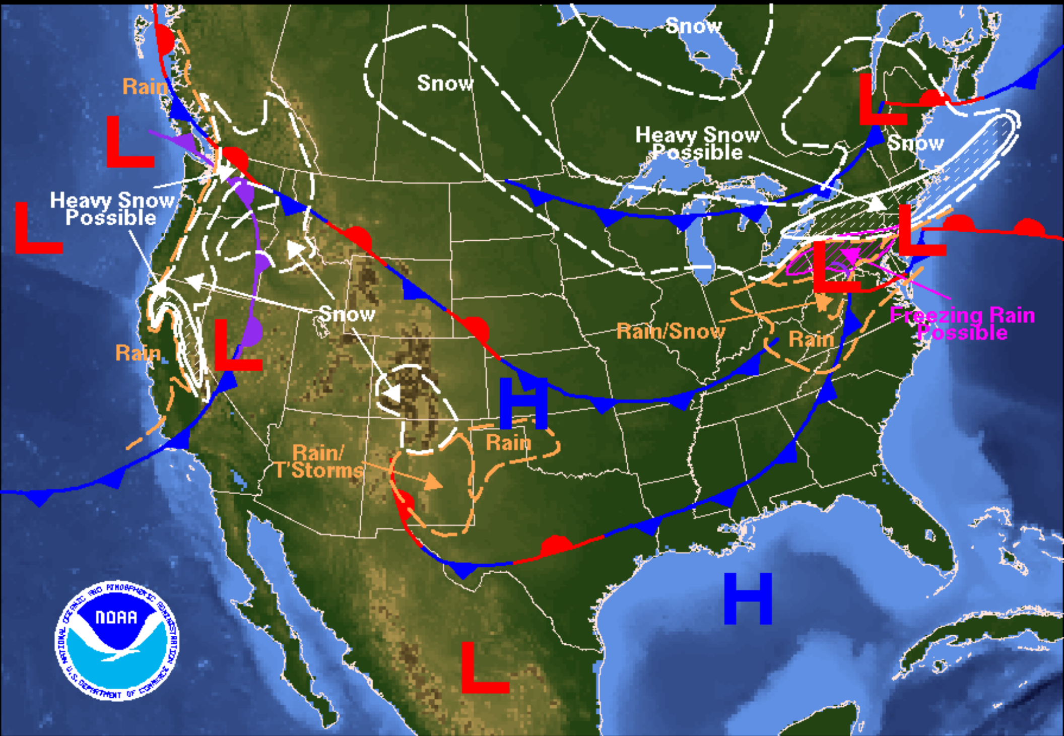
Weather Forecast for Thursday, March 02, 2006 DOC/NOAA/NWS/NCEP/Hydrometeorological Prediction Center Prepared by Otto based on HPC, SPC, and TPC forecasts.
