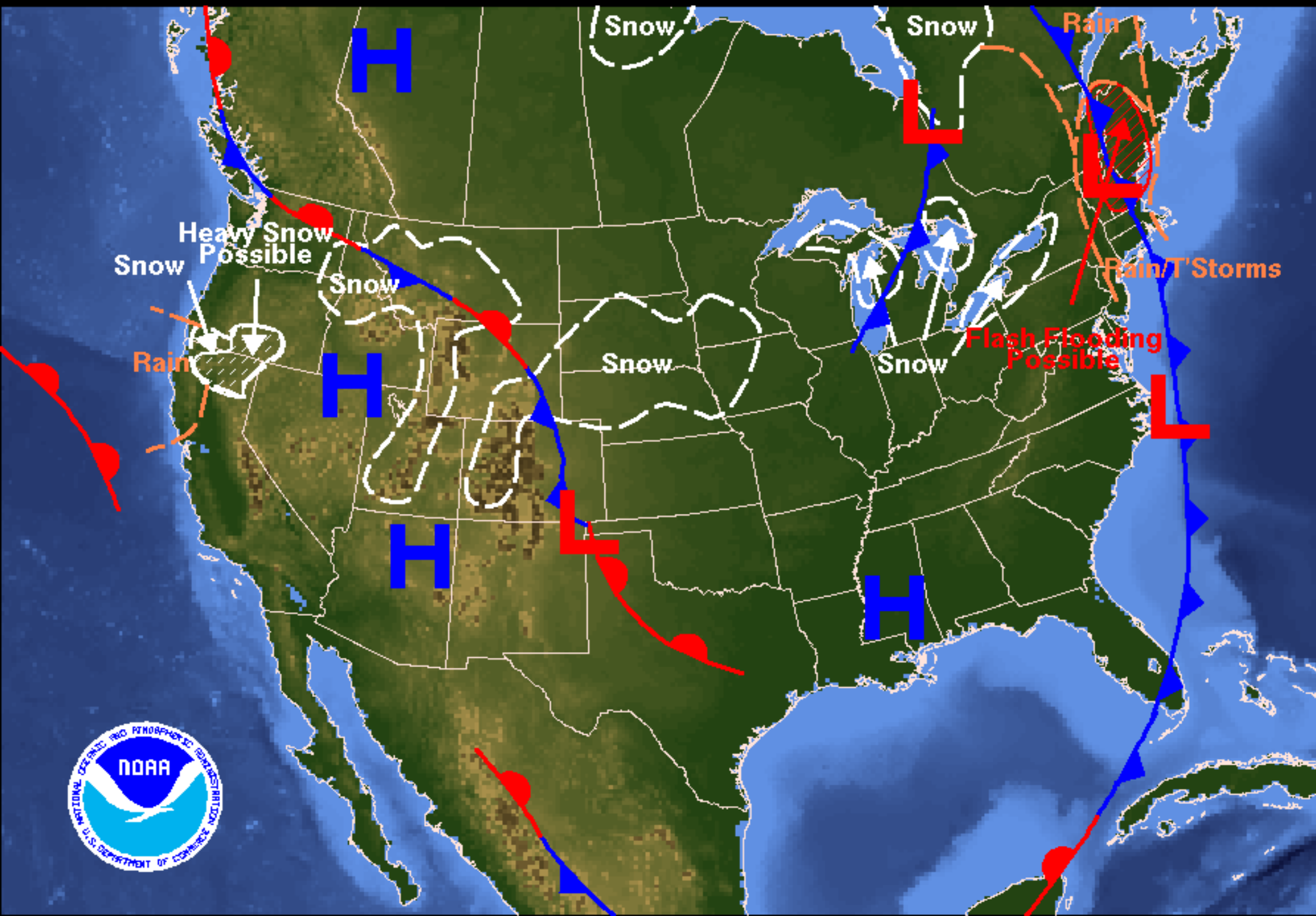
Weather Forecast for Wednesday, November 30, 2005 DOC/NOAA/NWS/NCEP/Hydrometeorological Prediction Center Prepared by Bell/Eckert based on HPC, SPC, and TPC forecasts.
