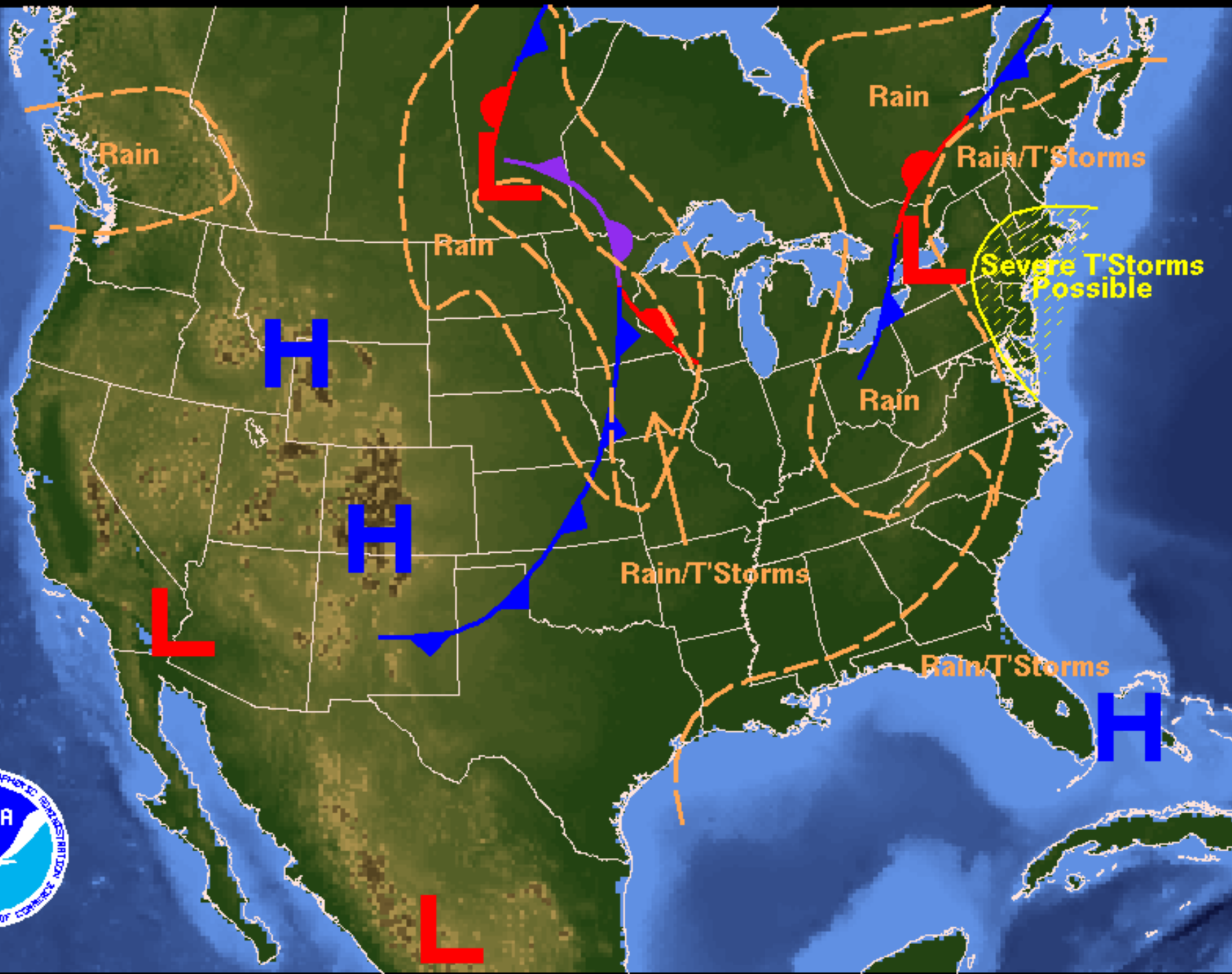
Weather Forecast for Wednesday, August 31, 2005 DOC/NOAA/NWS/NCEP/Hydrometeorological Prediction Center Prepared by Halbach/Korty based on HPC, SPC, and TPC forecasts.
