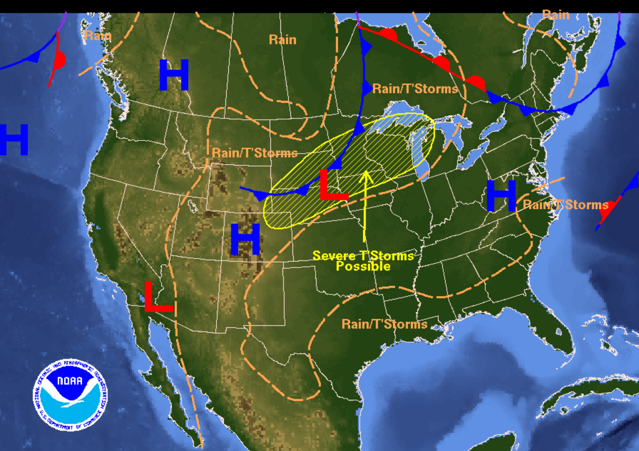
Weather Forecast for Wednesday, August 03, 2005 DOC/NOAA/NWS/NCEP/Hydrometeorological Prediction Center Prepared by Halbach/Sullivan based on HPC, SPC, and TPC forecasts.
