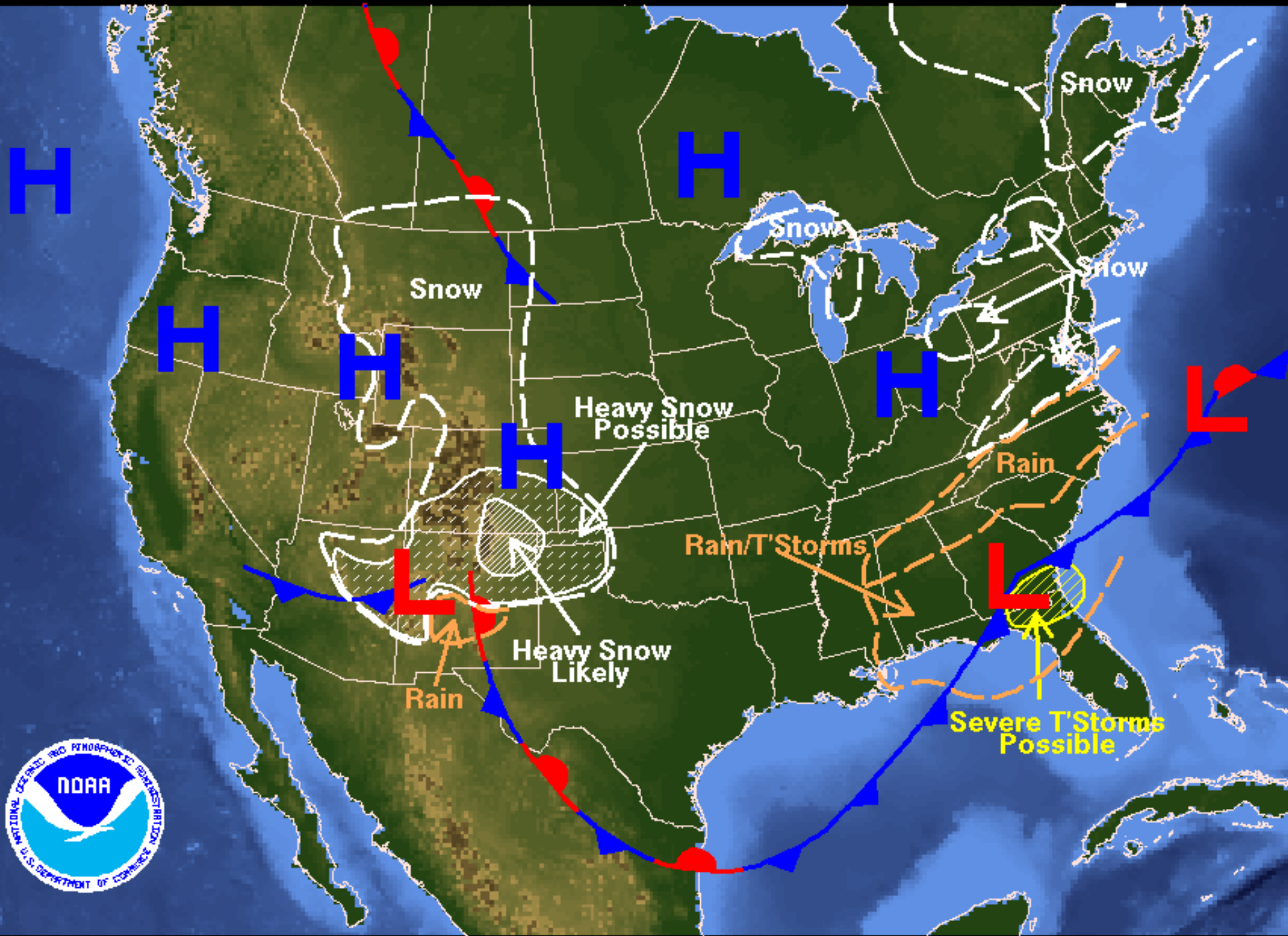
Weather Forecast for Monday, March 14, 2005 DOC/NOAA/NWS/NCEP/Hydrometeorological Prediction Center Prepared by Halbach/Sullivan based on HPC, SPC, and TPC forecasts.
