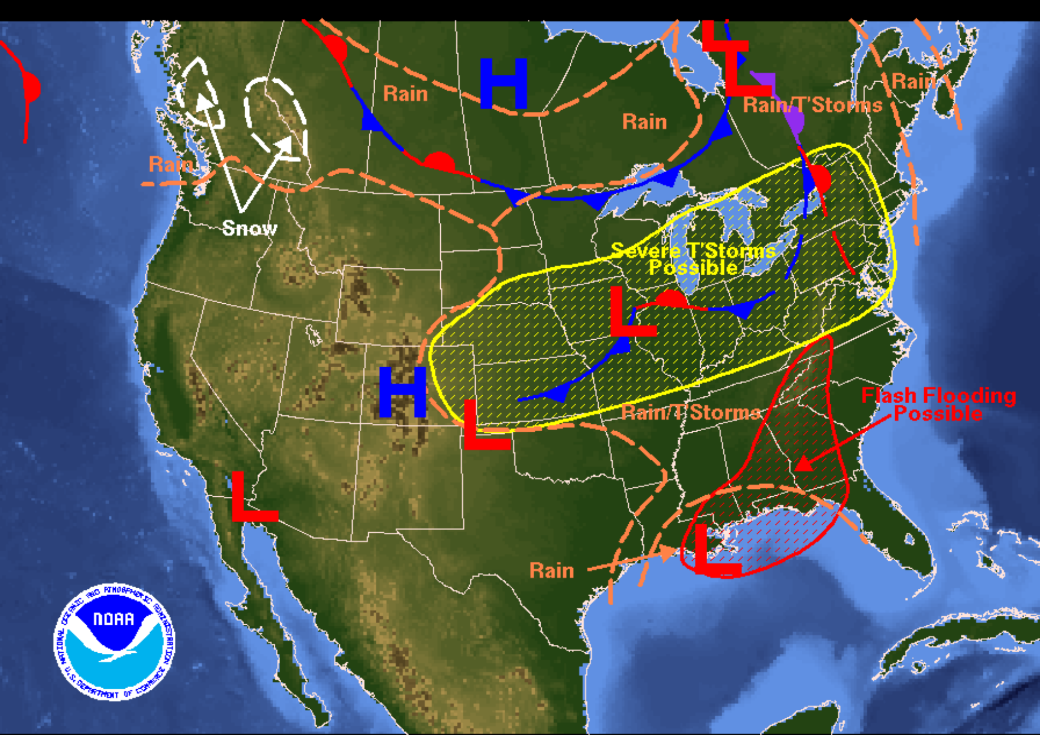
Weather Forecast for Monday, June 14, 2004 DOC/NOAA/NWS/NCEP/Hydrometeorological Prediction Center Prepared by Hatchett/Eckert based on HPC, SPC, and TPC forecasts.
