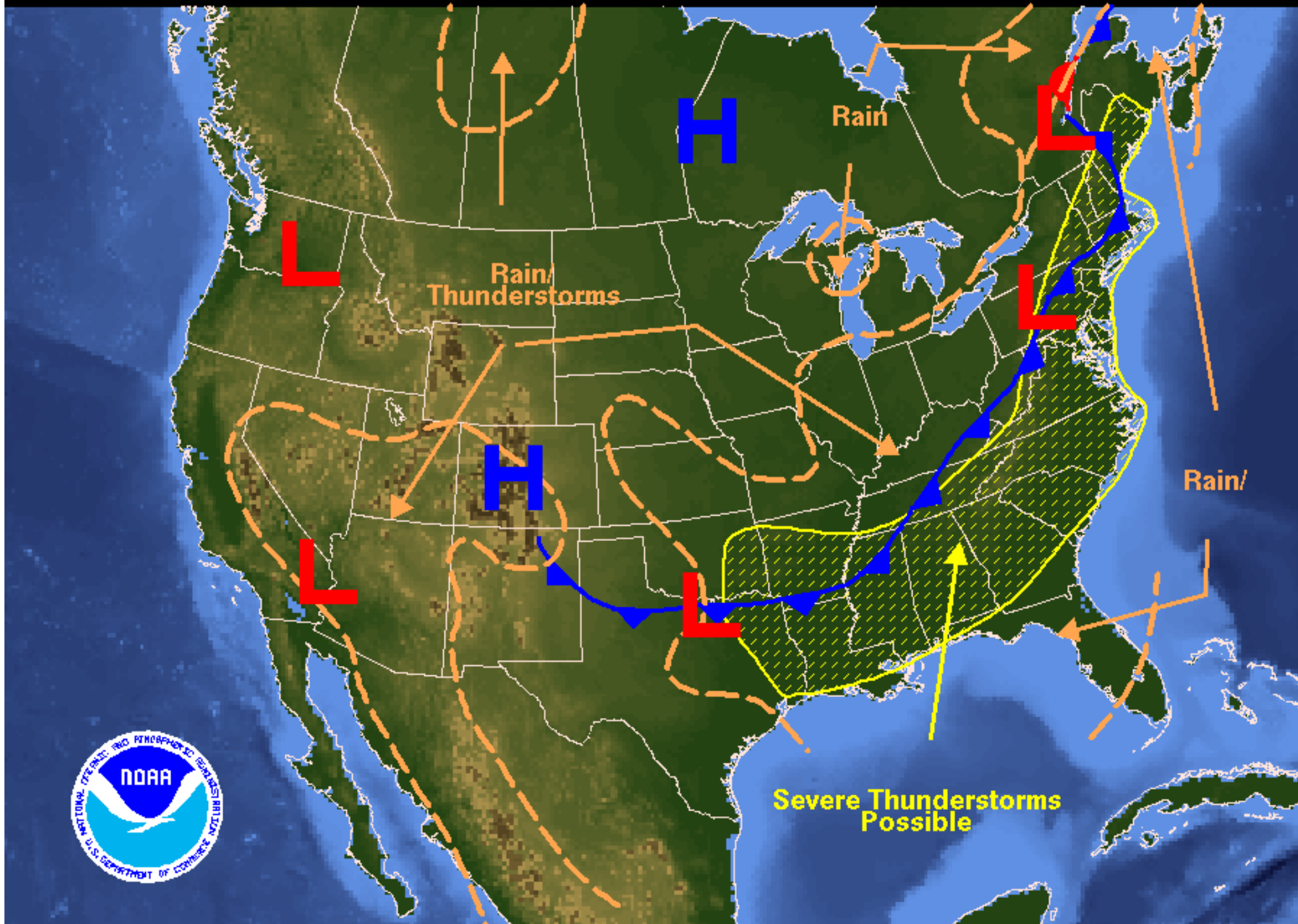
Weather Forecast for Tuesday, July 22, 2003 DOC/NOAA/NWS/NCEP/Hydrometeorological Prediction Center Prepared by JACKSON/KORTY based on HPC, SPC, and TPC forecasts.
