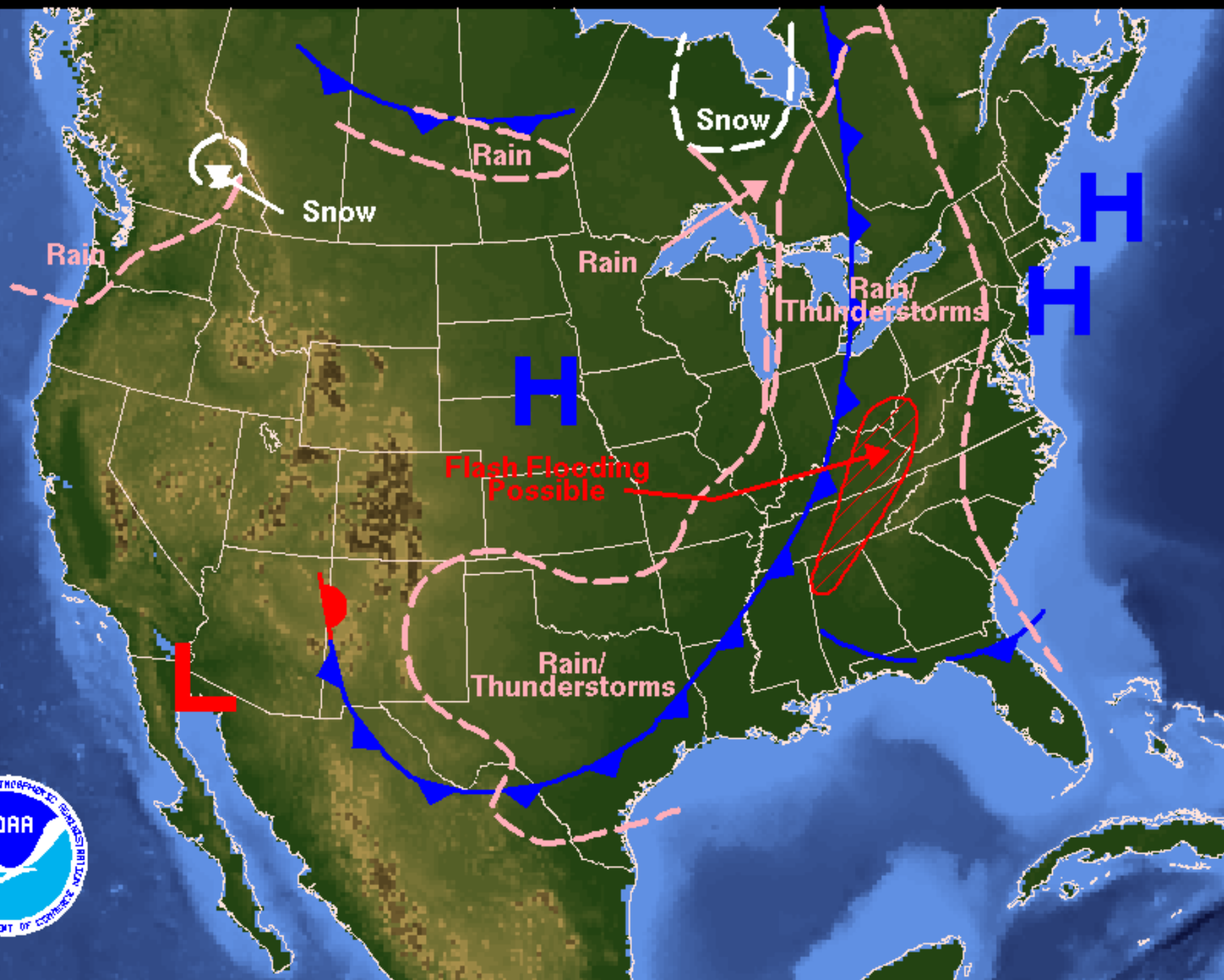
Weather Forecast for Tuesday May 20, 2003 DOC/NOAA/NWS/NCEP/Hydrometeorological Prediction Center Prepared by Hatchett/Junker based on HPC, SPC, and TPC forecasts.
