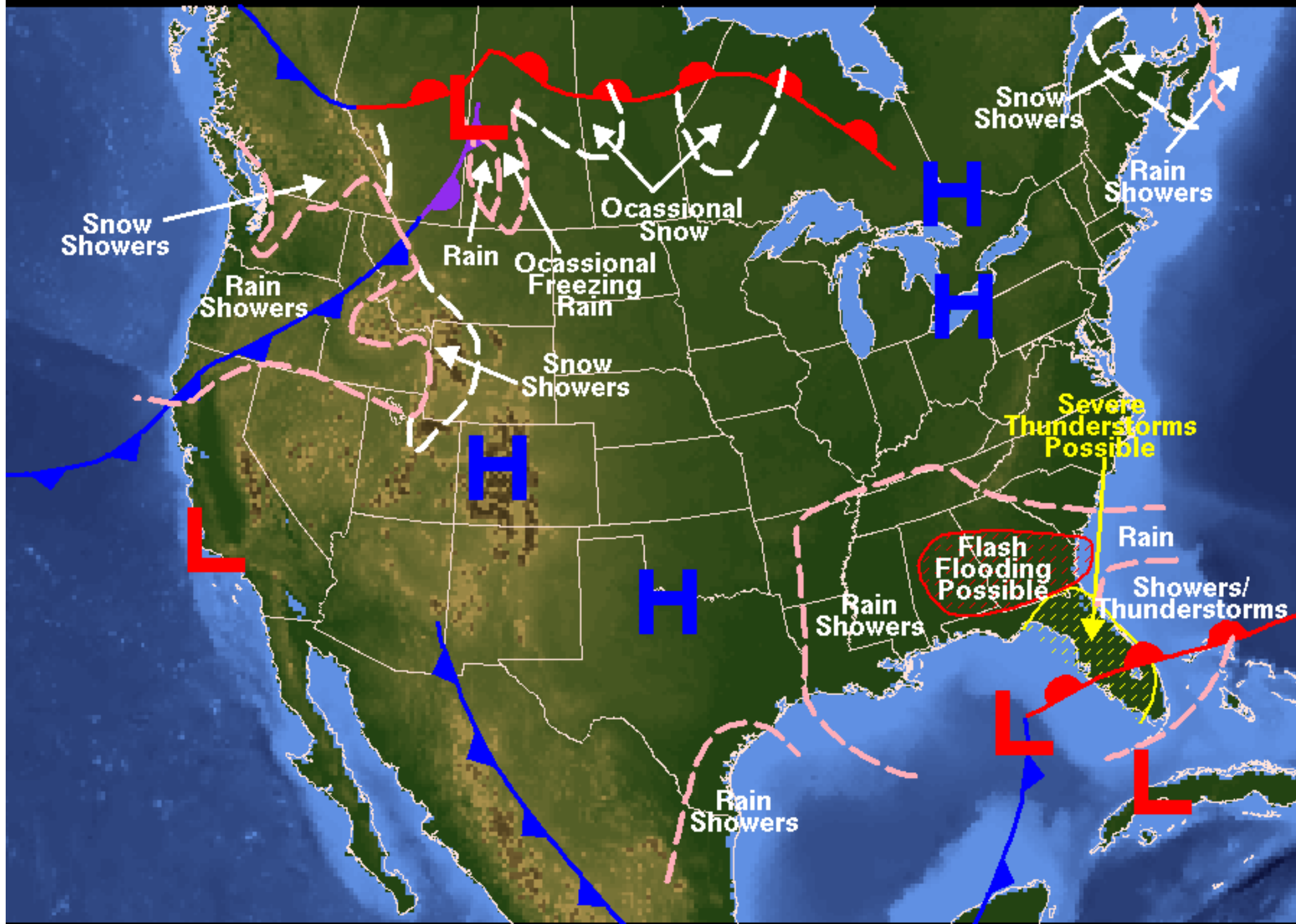
Weather Forecast for Monday, March 19, 2001 Prepared by HATCHETT/ECKERT DOC/NOAA/NWS/NCEP/Hydrometeorological Prediction Center
