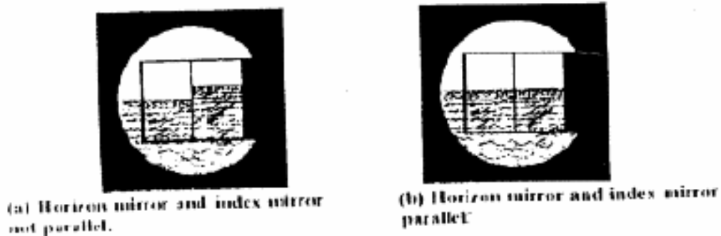
FIGURE 8-6 ADJUSTING THE SEXTANT - INDEX ERROR
