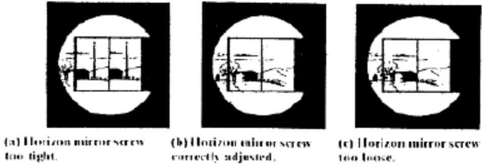
FIGURE 8-5 ADJUSTING THE SEXTANT - HORIZON MIRROR
