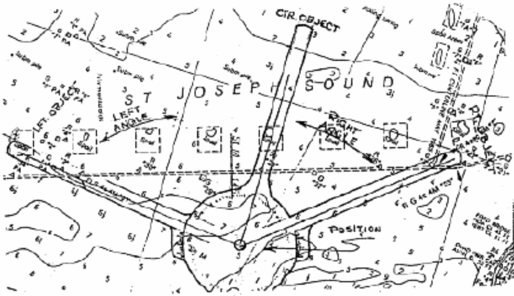
FIGURE 8-10 THREE-ARM PROTRACTOR - PLOTTING A THREE-POINT FIX
