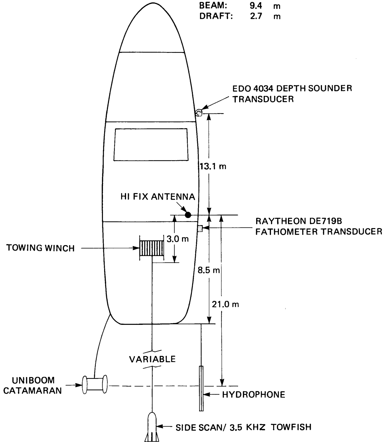
Project: EASTERN GULF OF MEXICO Project No. 41069 GEOPHYSICAL SURVEY VESSEL EQUIPMENT LAYOUT Fig. 3.1
