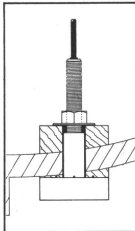
Thru-hull Mounting
