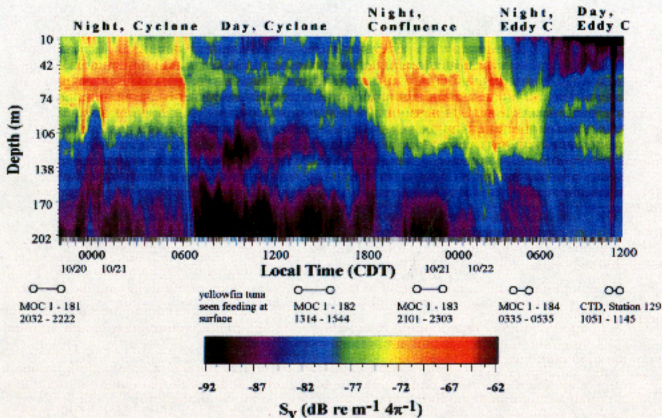
Figure 3.14. False color running plot of S_v collected along a north-south transect line from the MOM region, through the cyclone, and into Loop Current Eddy C during the late summer 1996 cruise. Depth is shown on the y-axis, while both time and location are changing along the x-axis. Periods of time corresponding to 1\text{ m}^2 MOCNESS tows and other events of interest are indicated below the x-axis. Reds and yellows on the plot indicate higher S_v , while blue and black colors indicate less intense returns. Note that both a temporal signal (higher S_v at night than in the daytime) and also a spatial signal (higher S_v in the cyclone than in the anticyclonic Eddy C) are evident.
