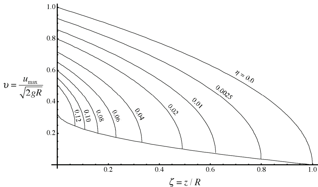
Figure 6-7 Maximum flow velocity of depth, d , at the ground elevation, z , and maximum runup elevation, R . The bottom curve represents the lower limit of maximum flow velocity.
