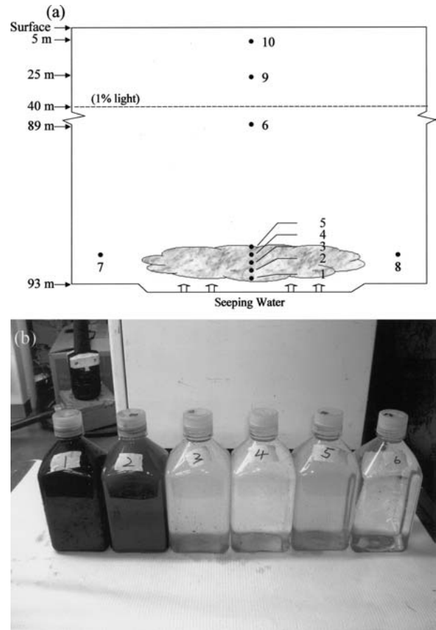
Figure 5. Generalized schematic cross-sectional diagram of the water column features and sampling sites over the Isolated Sinkhole environment (a) including the deep water nepheloid-like plume layer (near-bottom shaded area, samples 1 through 5), background deep lake water flanking samples (samples 6 through 8), background surface lake water (samples 9 and 10). Dotted line indicates depth of 1% surface sunlight (photosynthetically active radiation) penetration and a break in the water column between surface and near-bottom deep water. Photograph of recently retrieved samples collected in 1 l polycarbonate bottles (samples 1 through 6) showing dark coloration in sinkhole plume water samples 1 and 2 (b). Bottle numbers in b correspond with sample numbers in a.
