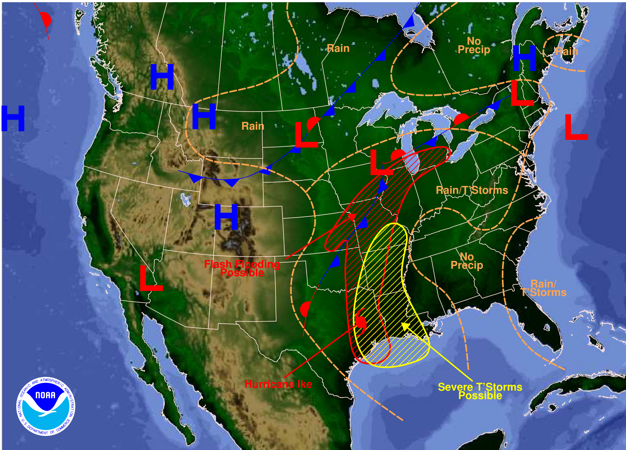
Weather Forecast for Saturday, September 13, 2008 DOC/NOAA/NWS/NCEP/Hydrometeorological Prediction Center Prepared by Kost based on HPC, SPC, and TPC forecasts.
