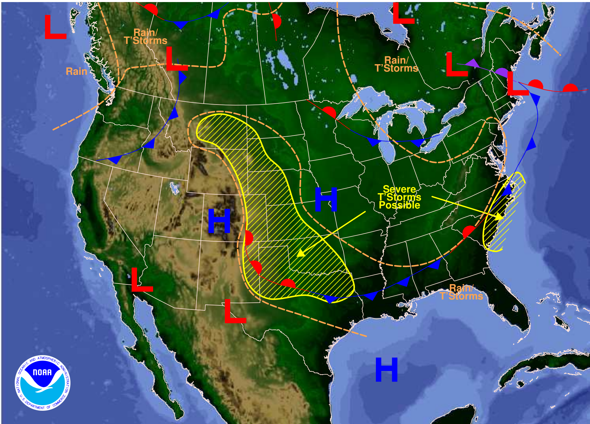
Weather Forecast for Tuesday, June 17, 2008 DOC/NOAA/NWS/NCEP/Hydrometeorological Prediction Center Prepared by Fracasso based on HPC, SPC, and TPC forecasts.
