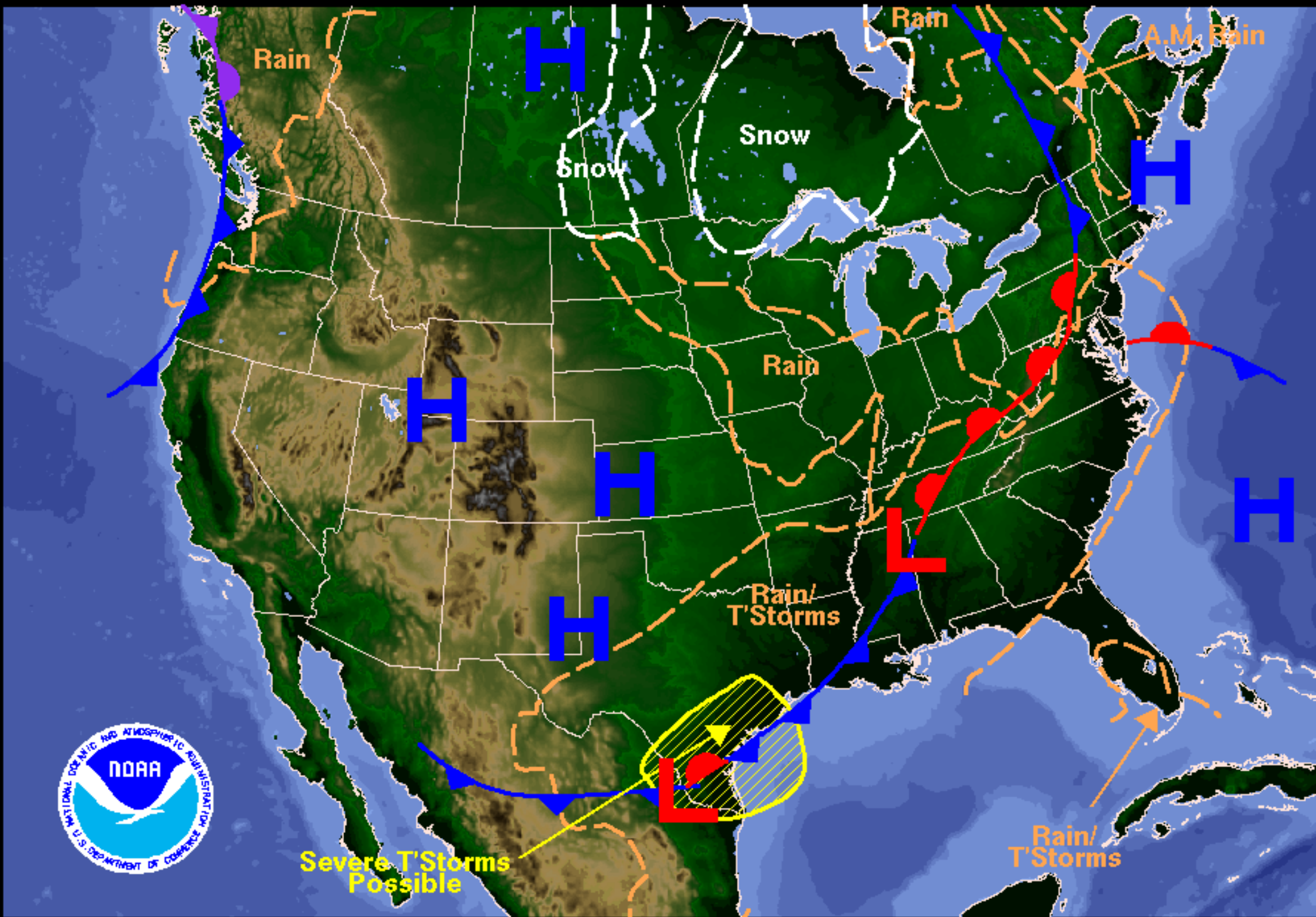
Weather Forecast for Sunday, April 27, 2008 DOC/NOAA/NWS/NCEP/Hydrometeorological Prediction Center Prepared by Rubin-Oster based on HPC, SPC, and TPC forecasts.
