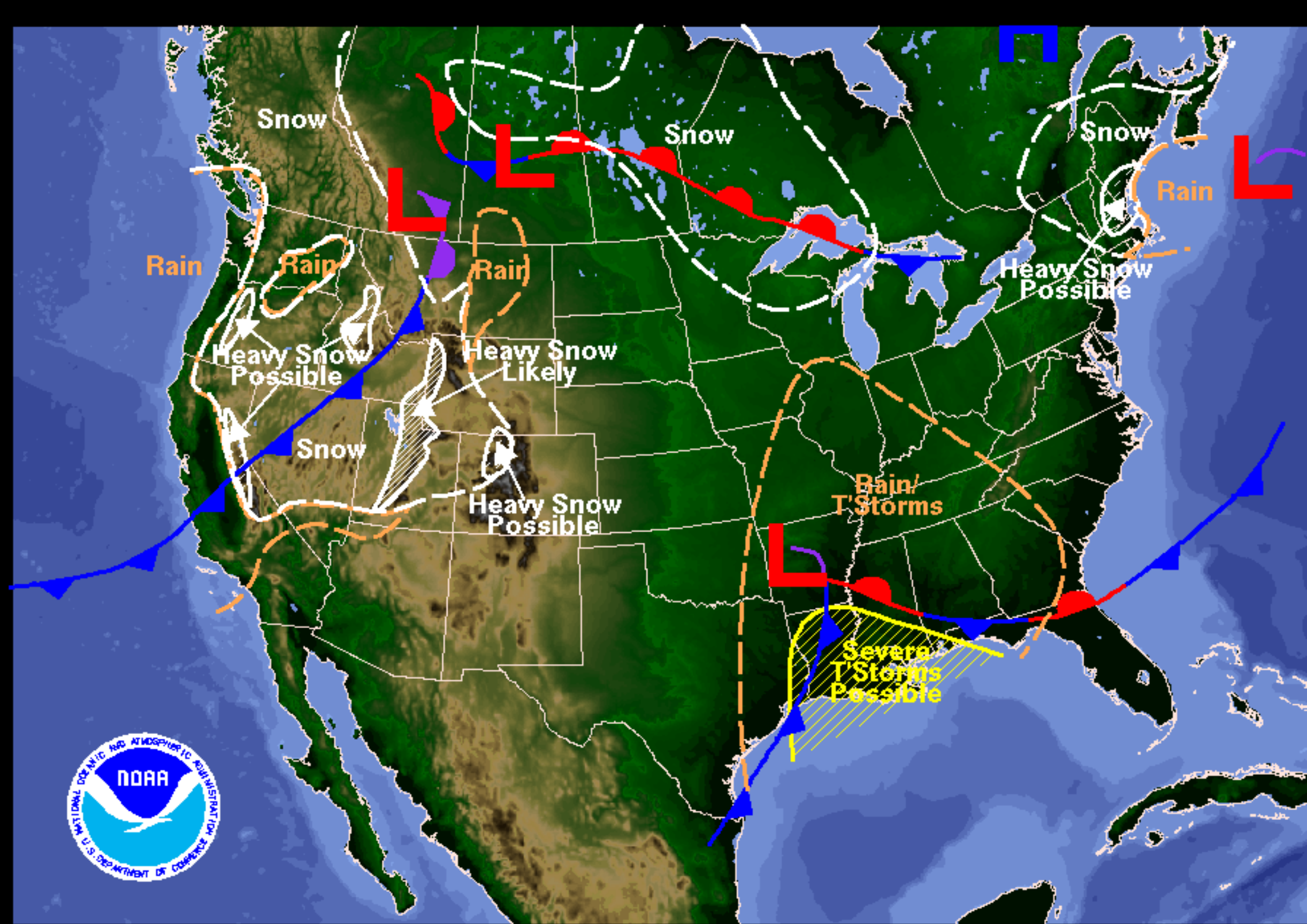
Weather Forecast for Thursday, December 20, 2007 DOC/NOAA/NWS/NCEP/Hydrometeorological Prediction Center Prepared by Roth based on HPC, SPC, and TPC forecasts.
