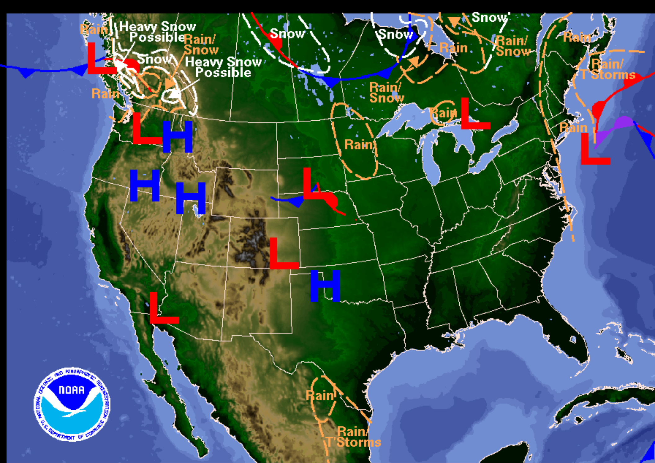
Weather Forecast for Saturday, November 03, 2007 DOC/NOAA/NWS/NCEP/Hydrometeorological Prediction Center Prepared by Kocin based on HPC, SPC, and TPC forecasts.
