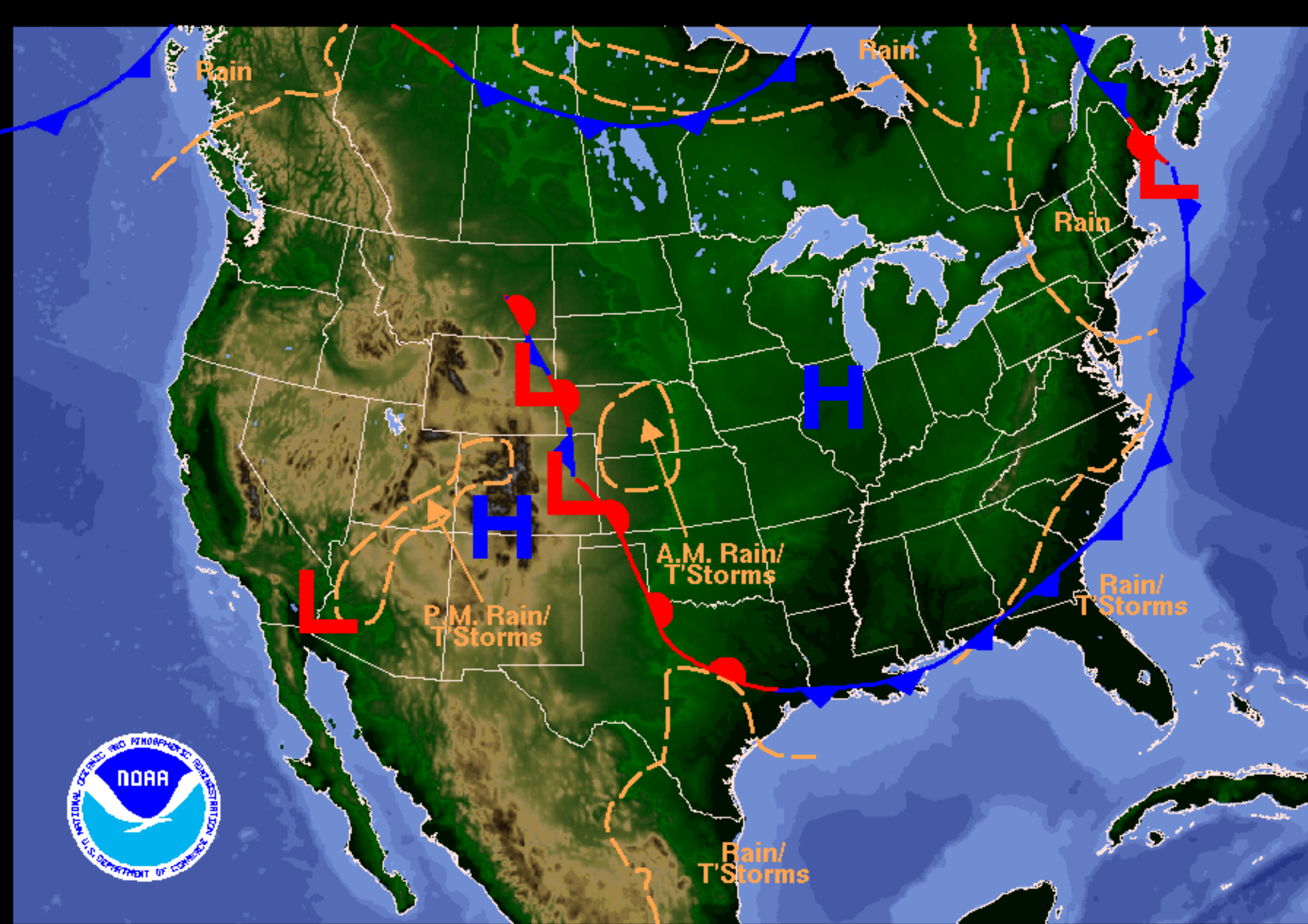
Weather Forecast for Saturday, September 15, 2007 DOC/NOAA/NWS/NCEP/Hydrometeorological Prediction Center Prepared by Rubin-Oster based on HPC, SPC, and TPC forecasts.
