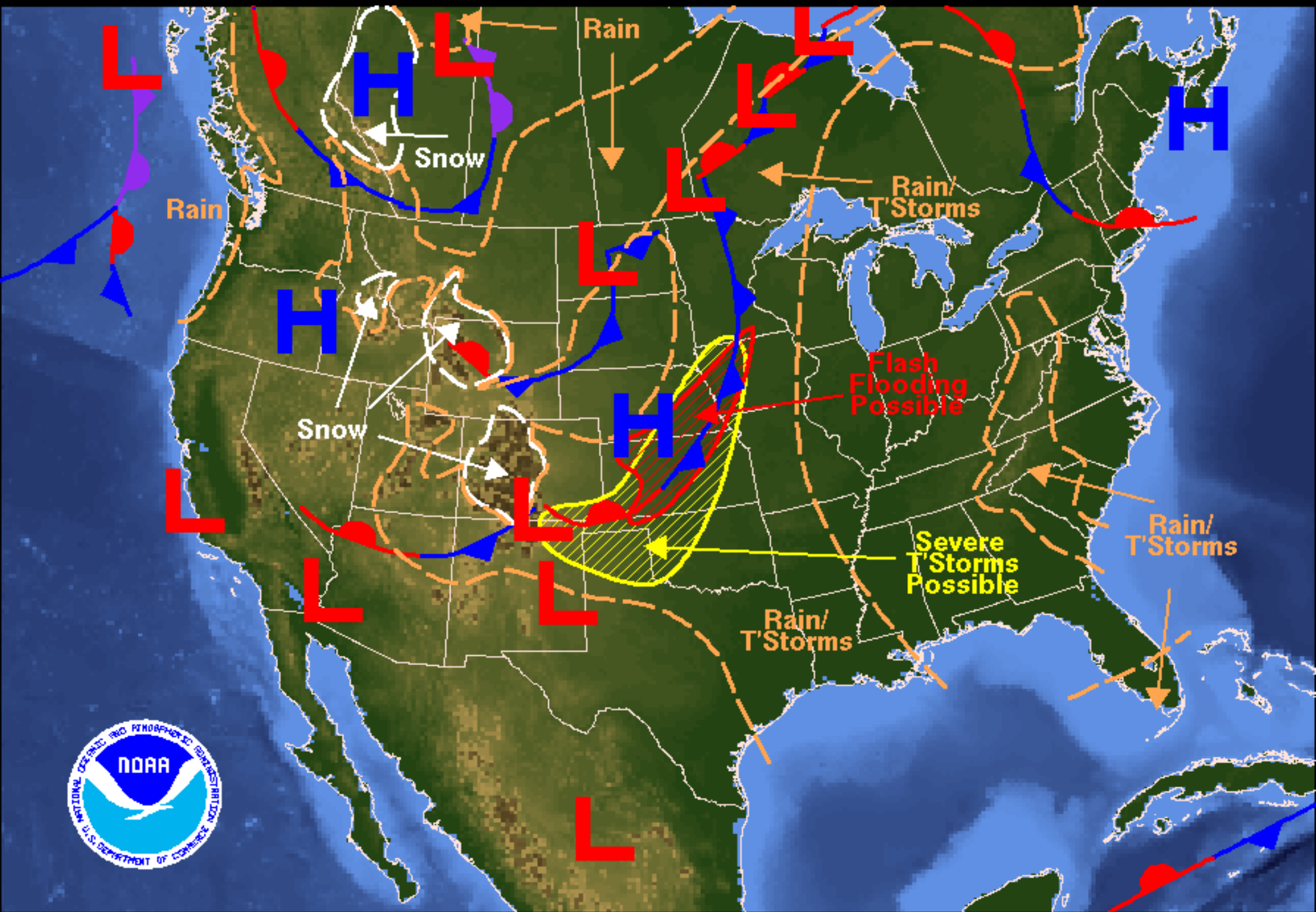
Weather Forecast for Wednesday, May 23, 2007 DOC/NOAA/NWS/NCEP/Hydrometeorological Prediction Center Prepared by Otto based on HPC, SPC, and TPC forecasts.
