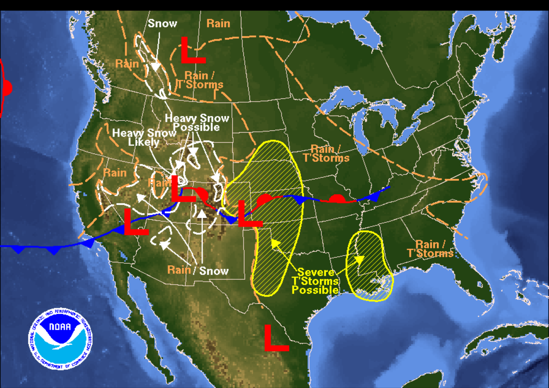
Weather Forecast for Friday, May 04, 2007 DOC/NOAA/NWS/NCEP/Hydrometeorological Prediction Center Prepared by Kong based on HPC, SPC, and TPC forecasts.
