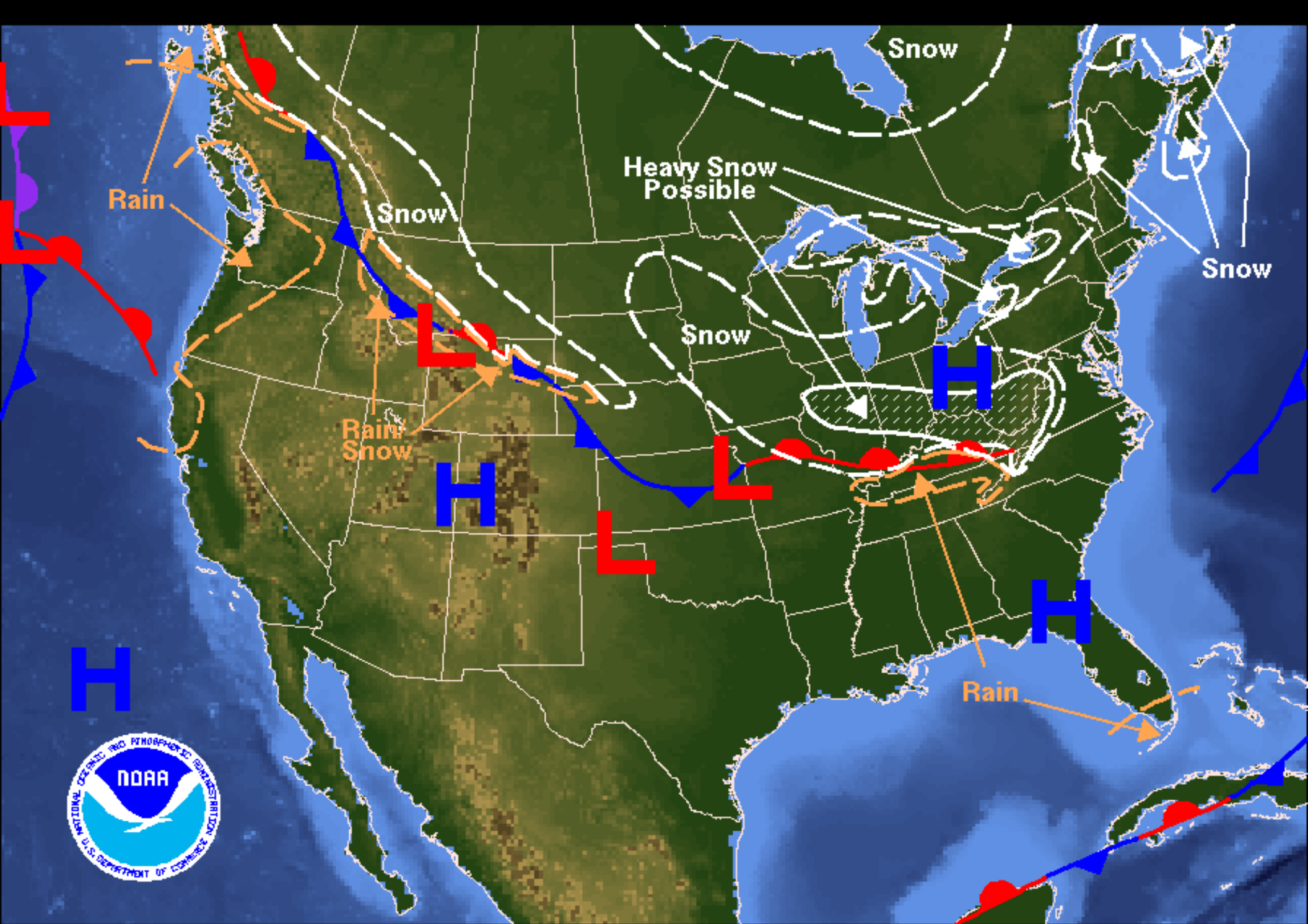
Weather Forecast for Tuesday, February 06, 2007 DOC/NOAA/NWS/NCEP/Hydrometeorological Prediction Center Prepared by Otto based on HPC, SPC, and TPC forecasts.
