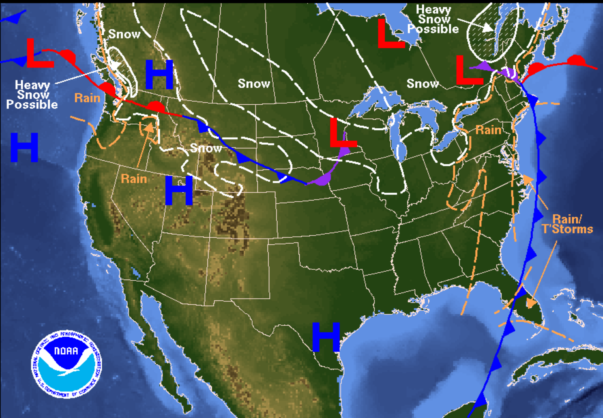
Weather Forecast for Monday, January 08, 2007 DOC/NOAA/NWS/NCEP/Hydrometeorological Prediction Center Prepared by Fracasso based on HPC, SPC, and TPC forecasts.
