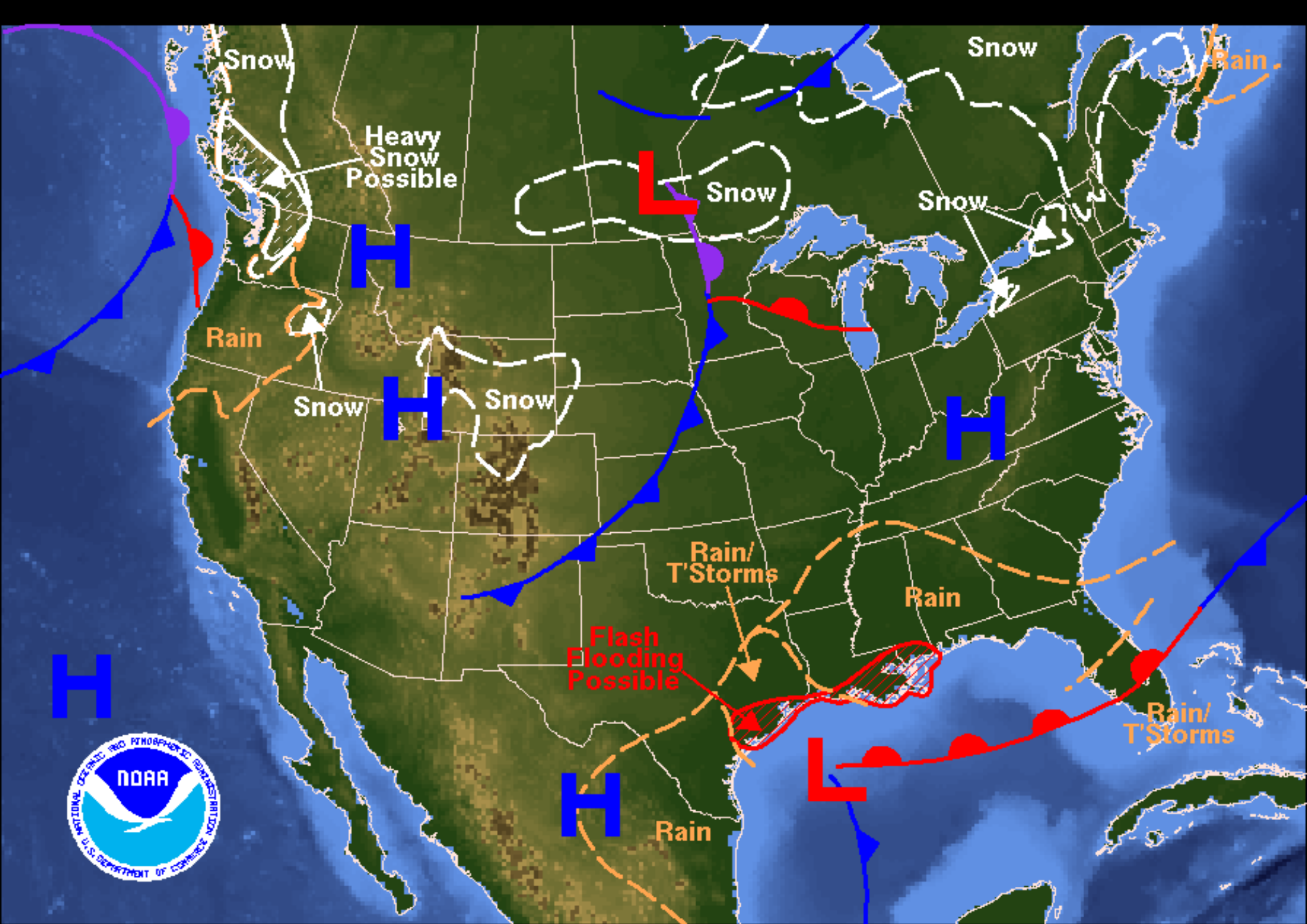
Weather Forecast for Sunday, December 24, 2006 DOC/NOAA/NWS/NCEP/Hydrometeorological Prediction Center Prepared by Trimarco based on HPC, SPC, and TPC forecasts.
