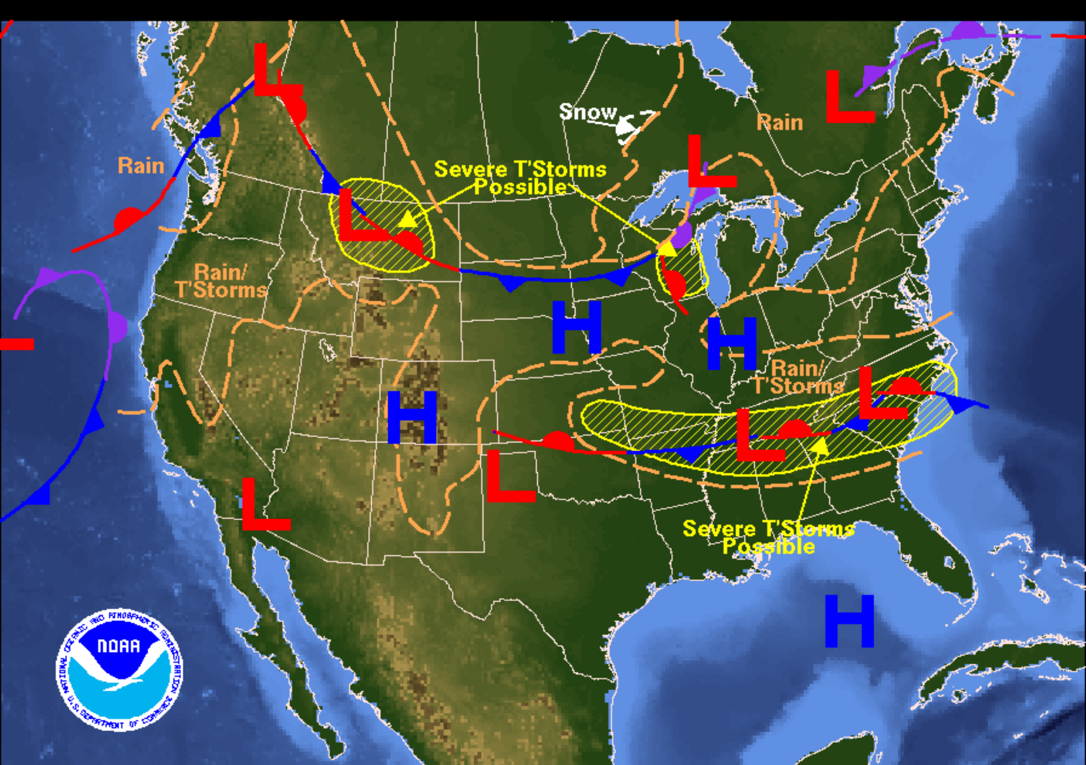
Weather Forecast for Saturday, May 20, 2006 DOC/NOAA/NWS/NCEP/Hydrometeorological Prediction Center Prepared by Fries based on HPC, SPC, and TPC forecasts.
