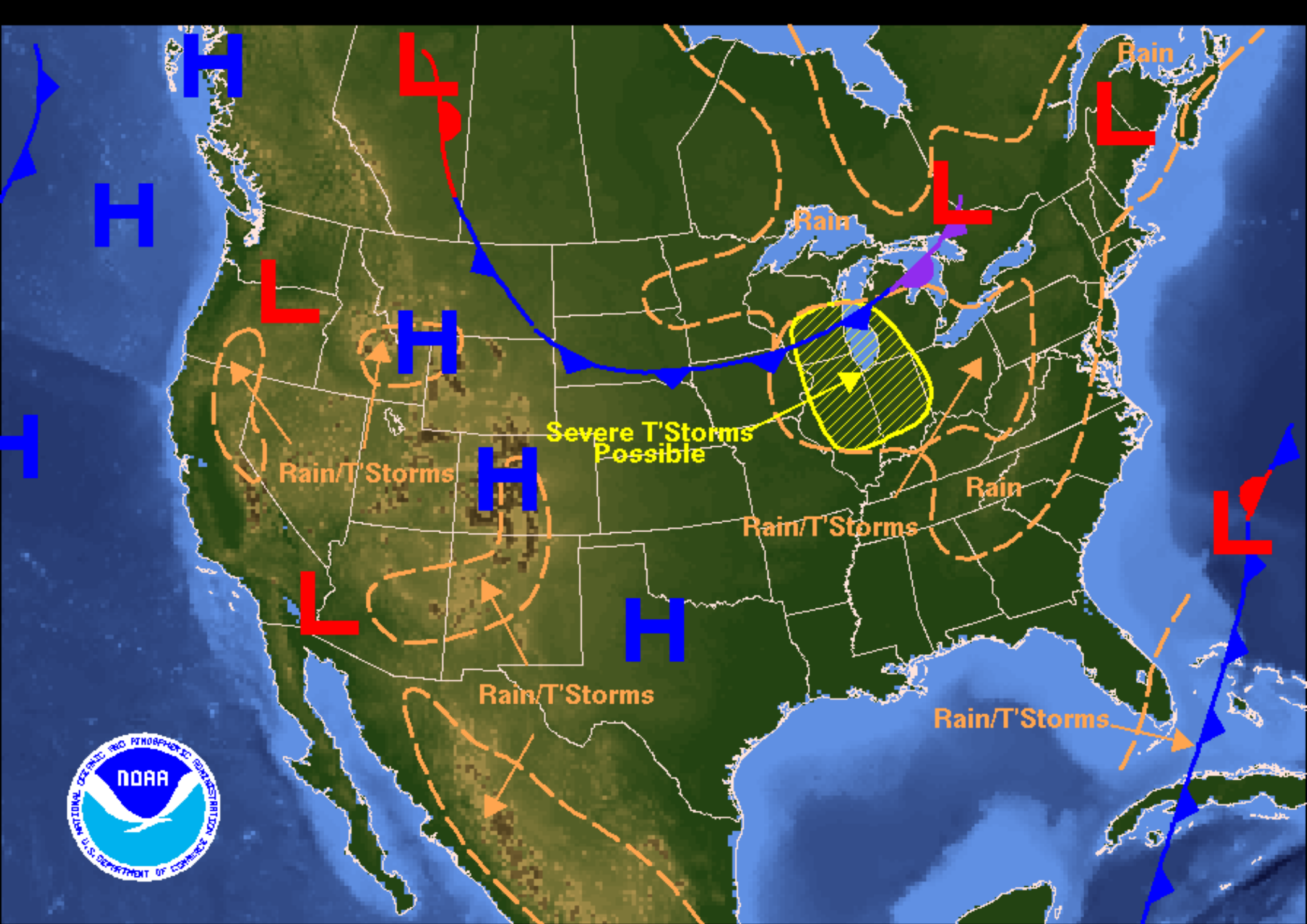
Weather Forecast for Wednesday, May 17, 2006 DOC/NOAA/NWS/NCEP/Hydrometeorological Prediction Center Prepared by Bell based on HPC, SPC, and TPC forecasts.
