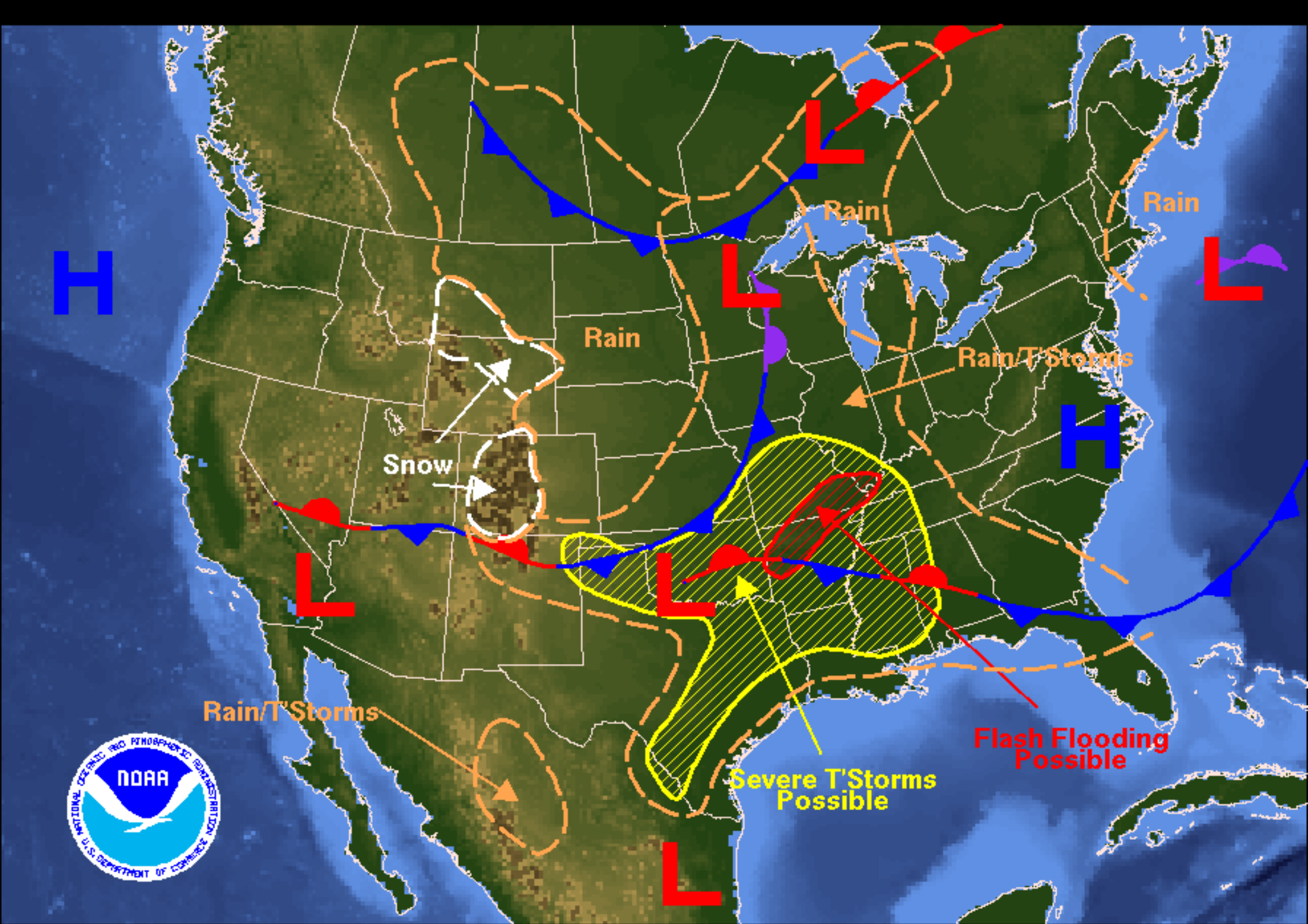
Weather Forecast for Tuesday, May 09, 2006 DOC/NOAA/NWS/NCEP/Hydrometeorological Prediction Center Prepared by Otto based on HPC, SPC, and TPC forecasts.
