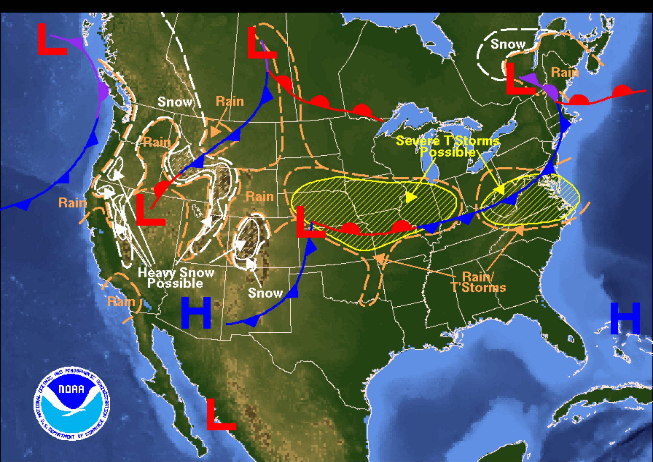
Weather Forecast for Saturday, April 15, 2006 DOC/NOAA/NWS/NCEP/Hydrometeorological Prediction Center Prepared by Fries based on HPC, SPC, and TPC forecasts.
