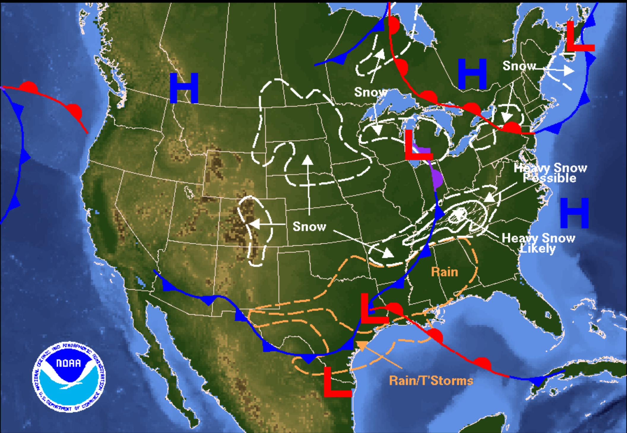
Weather Forecast for Friday, February 10, 2006 DOC/NOAA/NWS/NCEP/Hydrometeorological Prediction Center Prepared by Bell based on HPC, SPC, and TPC forecasts.
