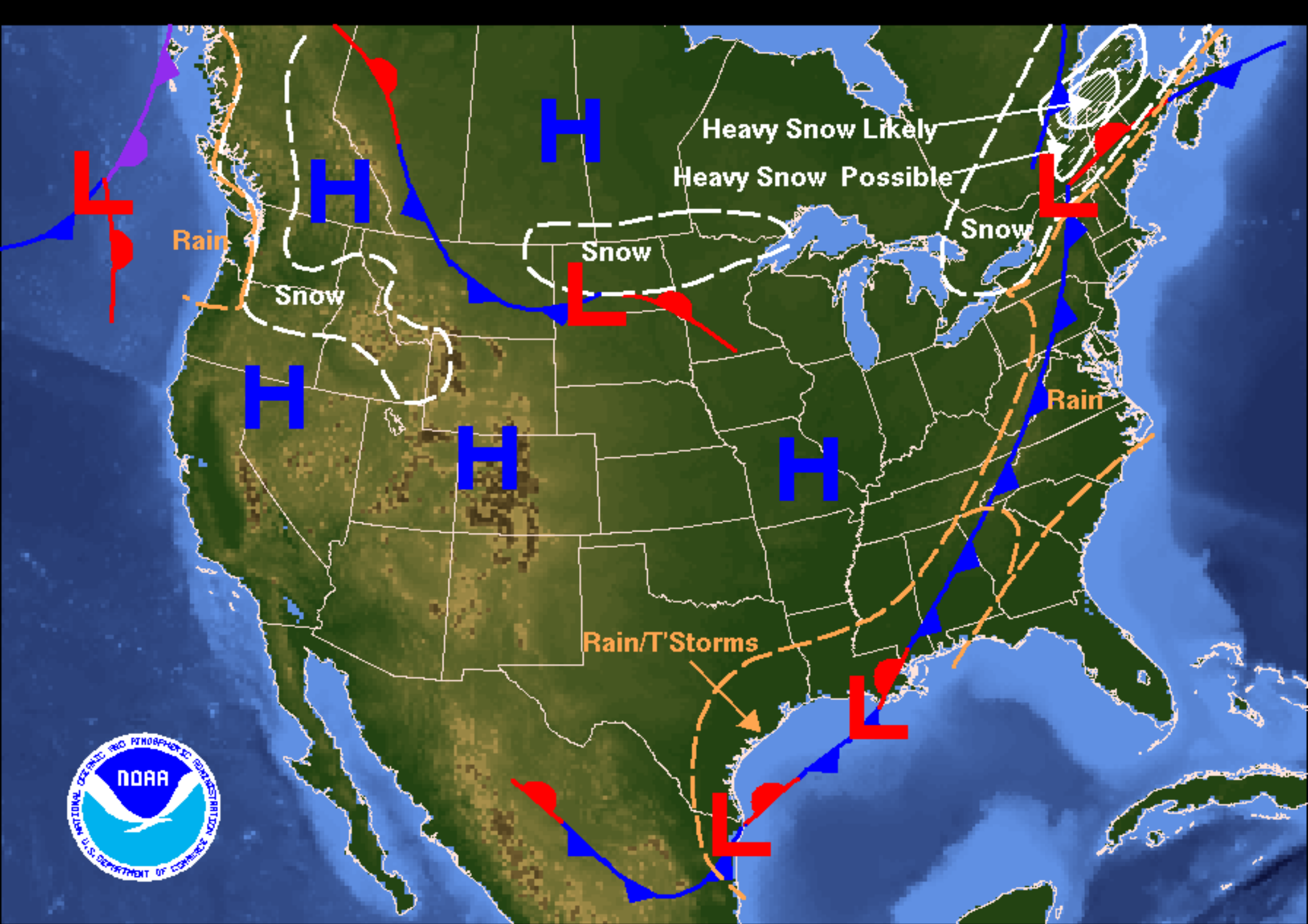
Weather Forecast for Saturday, January 21, 2006 DOC/NOAA/NWS/NCEP/Hydrometeorological Prediction Center Prepared by Szatanek based on HPC, SPC, and TPC forecasts.
