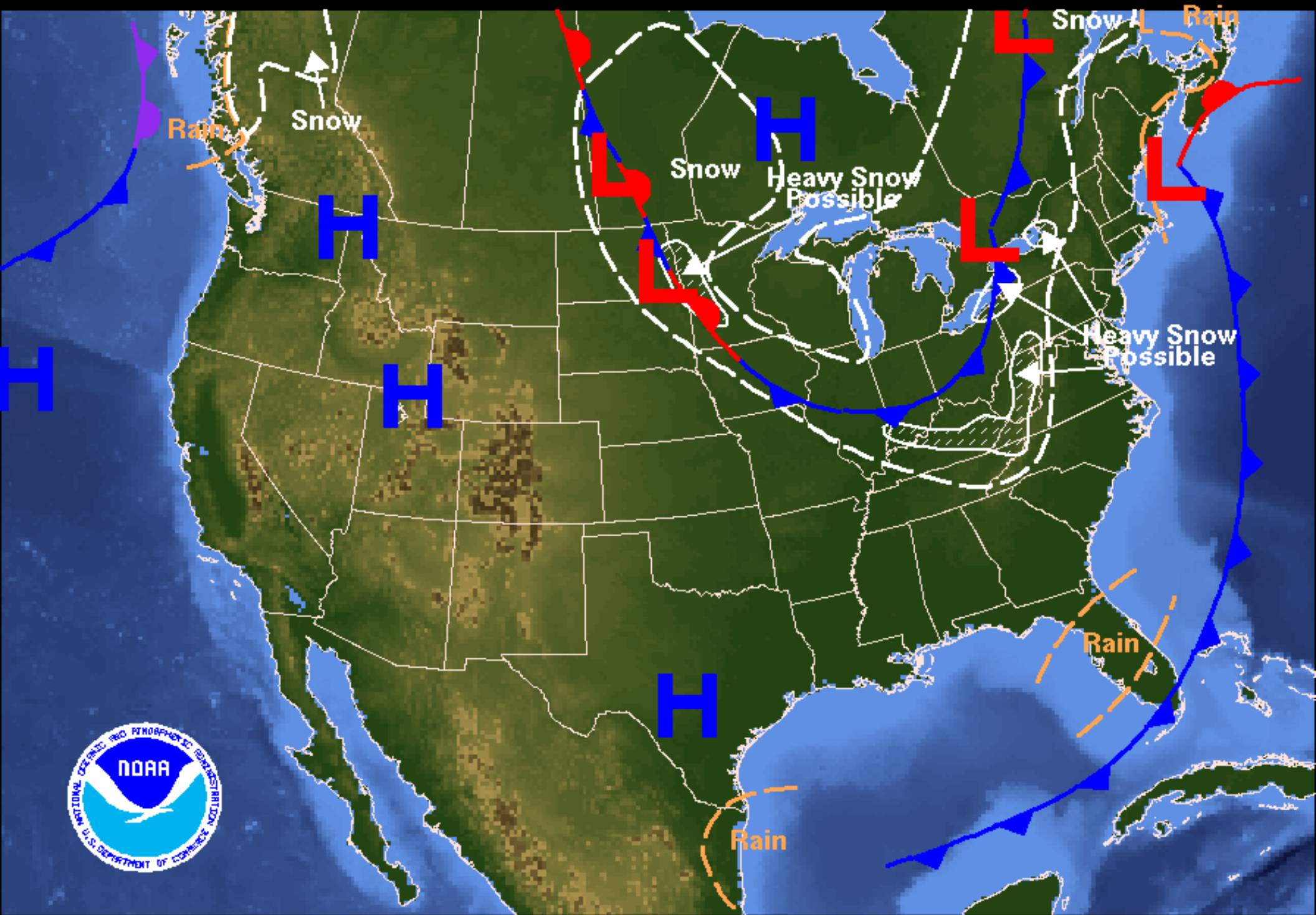
Weather Forecast for Sunday, December 11, 2005 DOC/NOAA/NWS/NCEP/Hydrometeorological Prediction Center Prepared by Fries based on HPC, SPC, and TPC forecasts.
