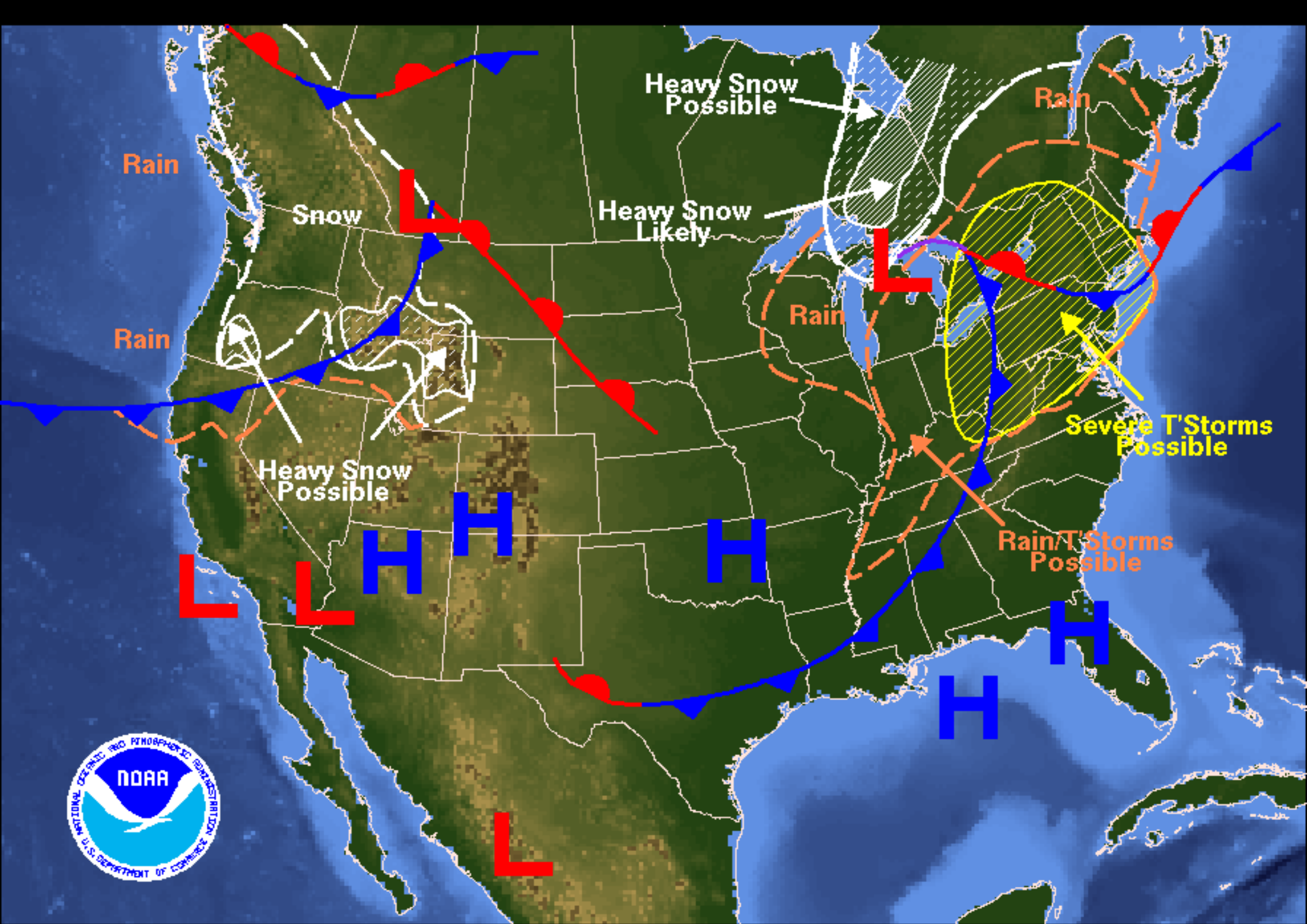
Weather Forecast for Sunday, November 06, 2005 DOC/NOAA/NWS/NCEP/Hydrometeorological Prediction Center Prepared by Bell/Korty based on HPC, SPC, and TPC forecasts.
