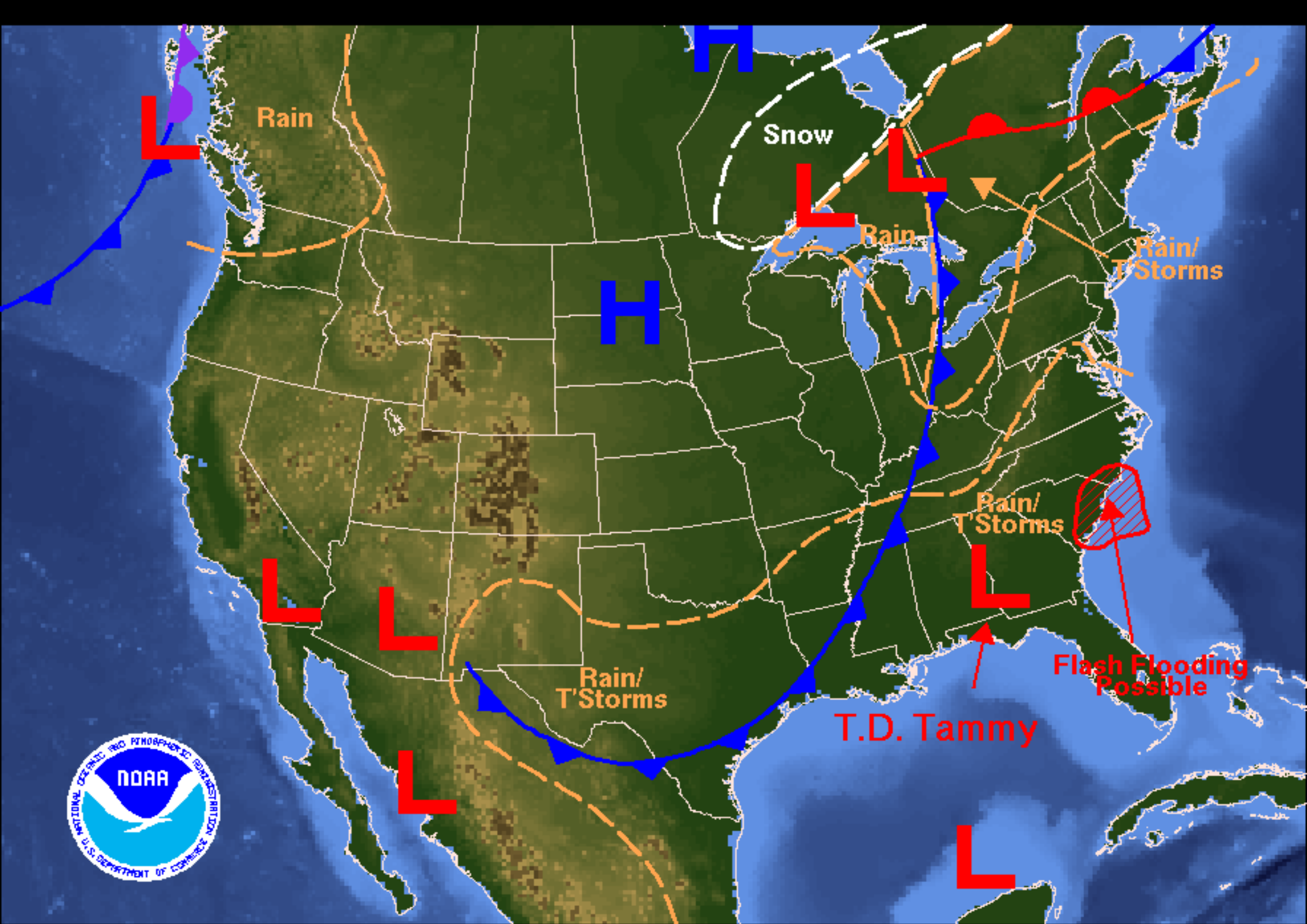
Weather Forecast for Thursday, October 06, 2005 DOC/NOAA/NWS/NCEP/Hydrometeorological Prediction Center Prepared by Szatane/Sullivan based on HPC, SPC, and TPC forecasts.
